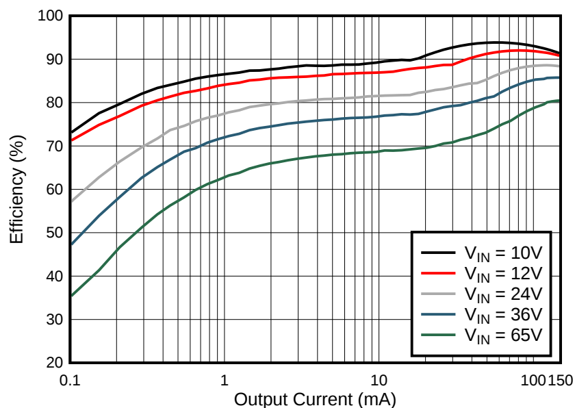
Figure 4. Converter Efficiency
