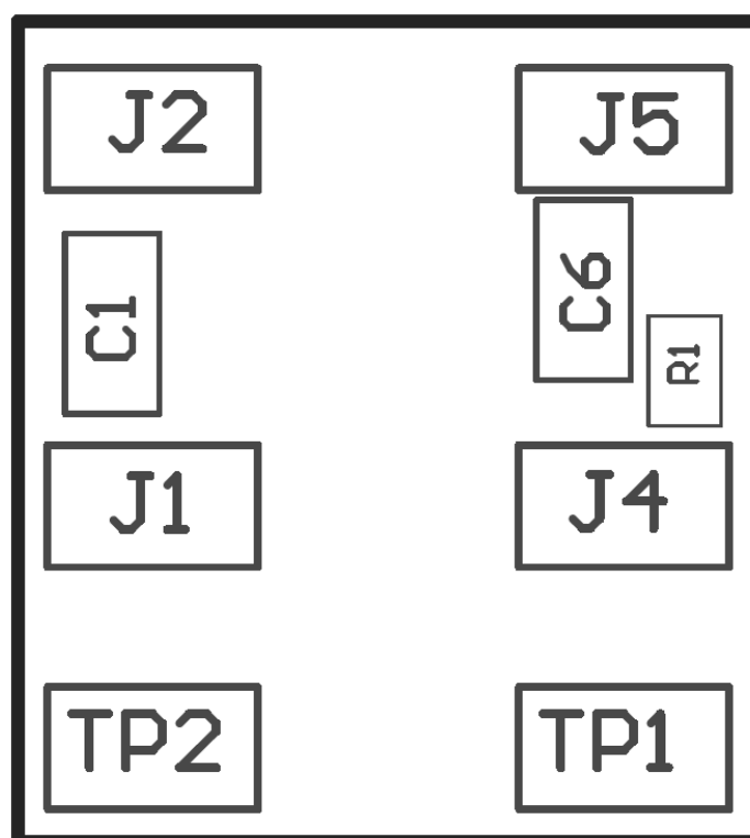
Figure 34. Bottom Assembly
