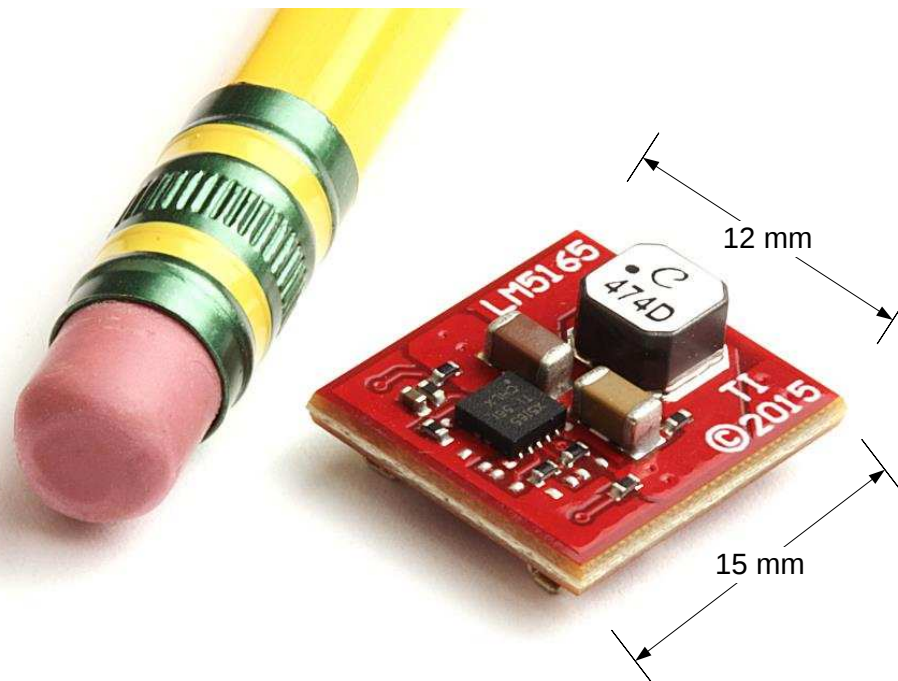
Figure 2. LM5165 EVM Photo
