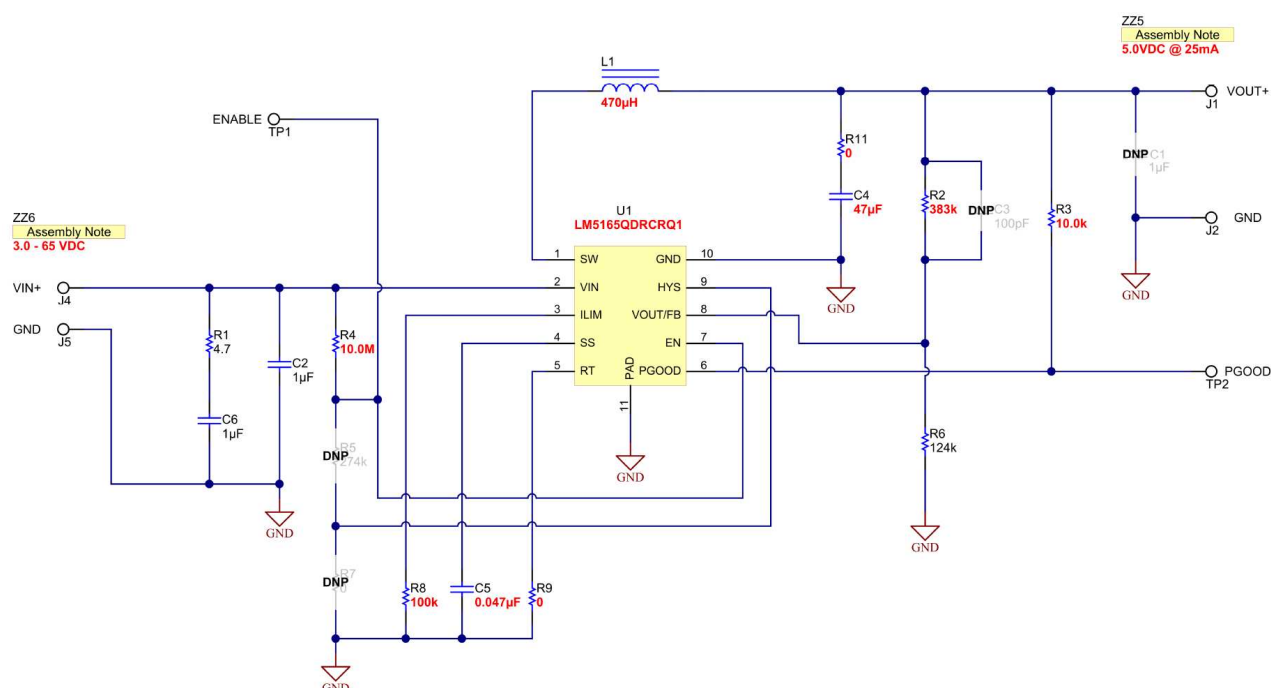
Figure 36. 5V, 25mA PFM Schematic (Adjustable Output Version)
