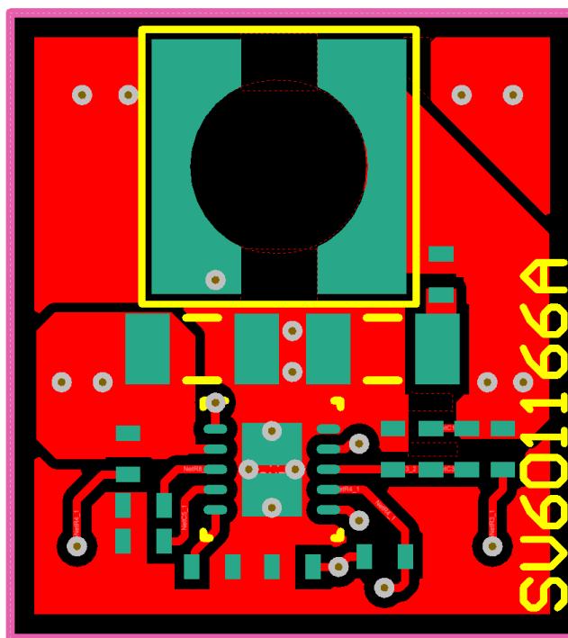
Figure 29. Top Copper (Top View)
