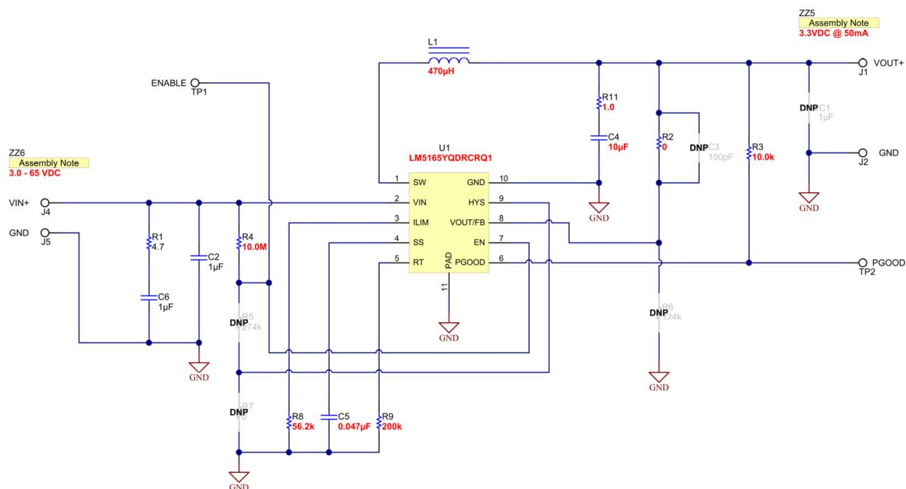
Figure 35. 3.3V, 50mA COT Schematic (Fixed 3.3V Output Version)
