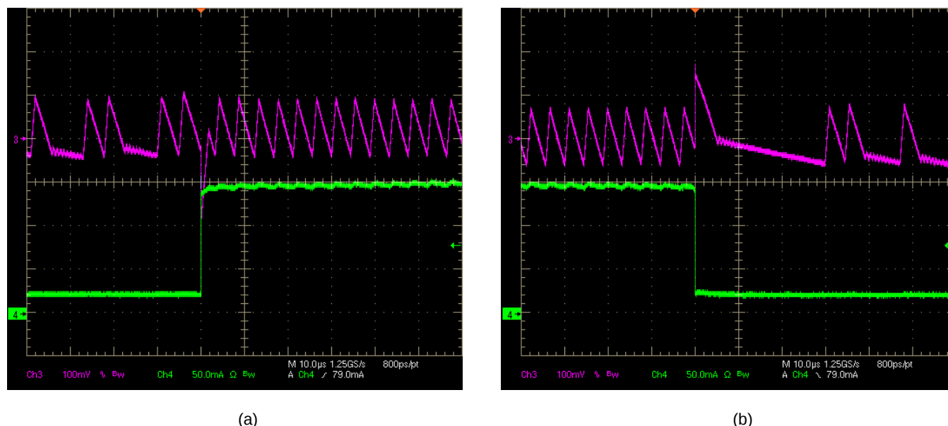
Figure 14. Load Transient Response, V_{IN} = 24\text{ V} , 20 mA to 150 mA at 2 A/μs; (a) Load-on transient, (b) Load-off transient
