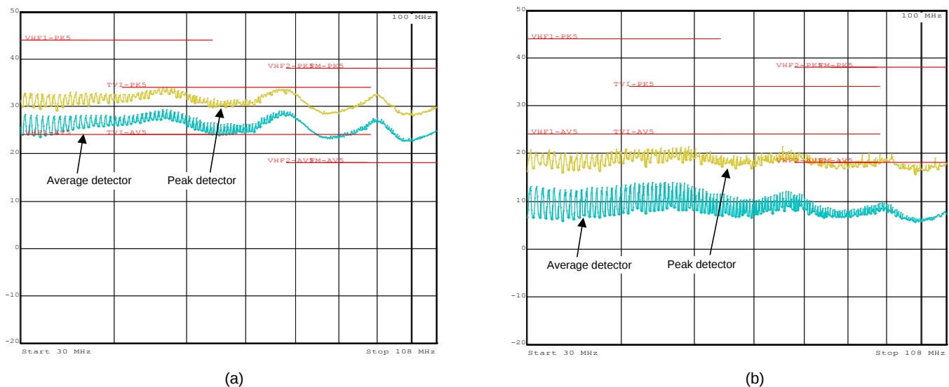
Figure 26. CISPR 25 Class 5 Conducted Emissions Plot, 30 MHz to 108 MHz, V_{IN} = 13.5 V, I_{OUT} = 100 mA, (a) Unfiltered, (b) Filtered
