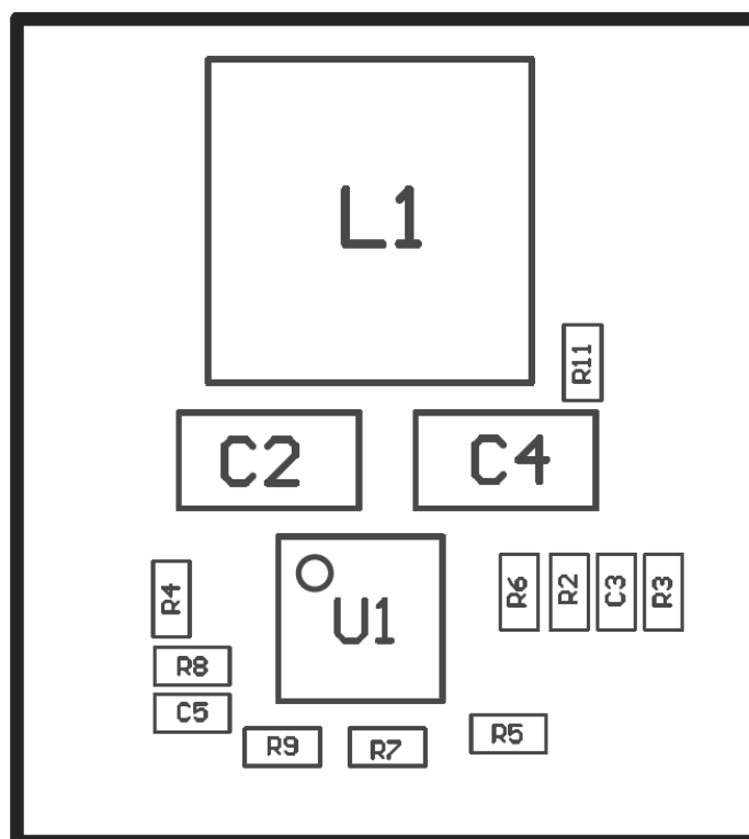
Figure 33. Top Assembly
