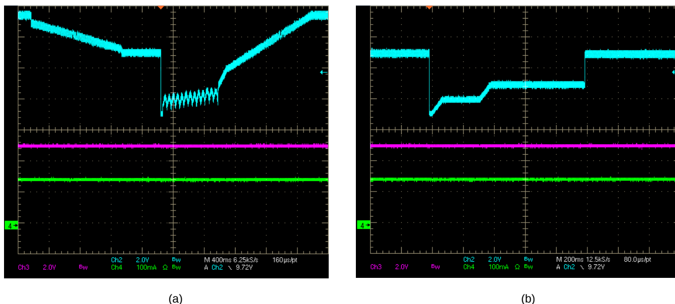
Figure 23. Typical automotive cold-crank input voltage transient; I_{OUT} = 150\text{ mA} ; (a) Profile 1, (b) Profile 2 (Ch2: V_{IN} , Ch3: V_{OUT} , Ch4: I_{OUT} )
