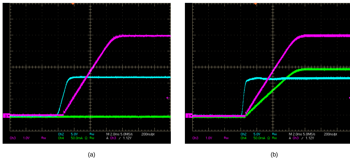
Figure 15. Startup: V_{IN} = 12\text{ V} ; (a) I_{OUT} = 0\text{ mA} , (b) I_{OUT} = 150\text{ mA} (Ch2: V_{IN} , Ch3: V_{OUT} , Ch4: I_{OUT} )
