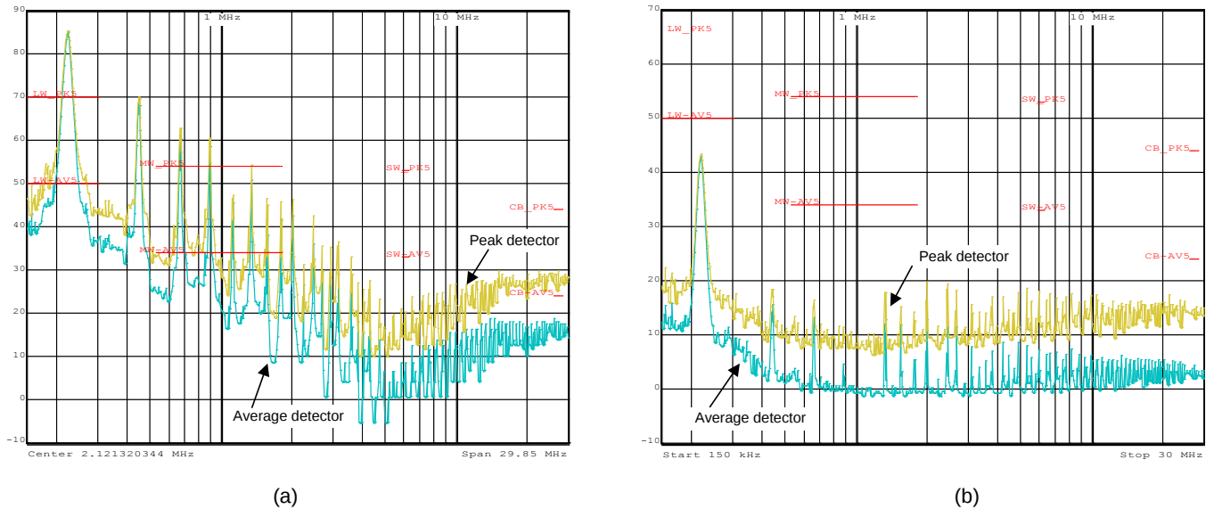
Figure 25. CISPR 25 Class 5 Conducted Emissions Plot, 150 kHz to 30 MHz, V_{IN} = 13.5 V, I_{OUT} = 100 mA, (a) Unfiltered, (b) Filtered
