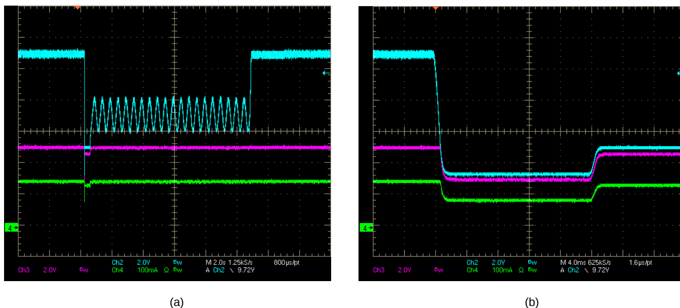
Figure 24. Typical automotive cold-crank input voltage transient; I_{OUT} = 150\text{ mA} ; (a) Profile 3, (b) Profile 3 zoomed to show dropout operation when V_{IN} < 5\text{ V} (Ch2: V_{IN} , Ch3: V_{OUT} , Ch4: I_{OUT} )
