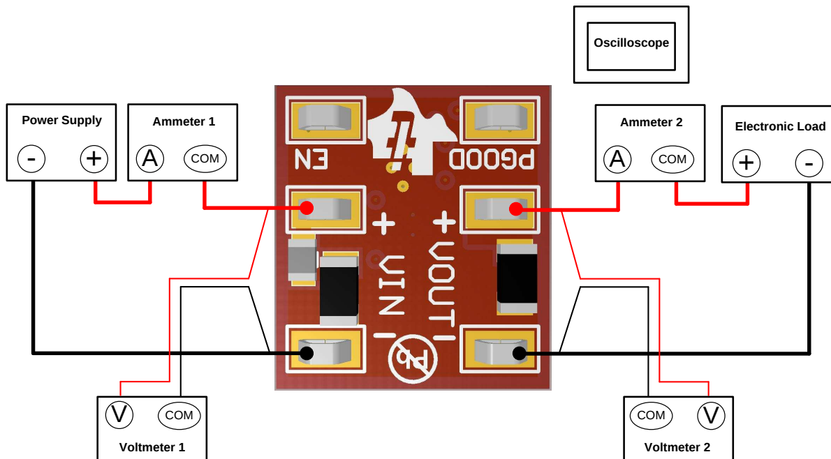
Figure 3. EVM Test Setup
