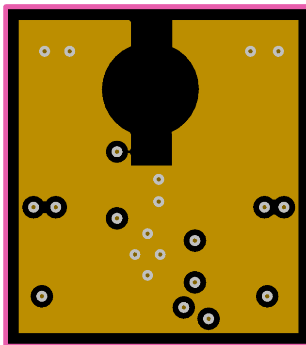
Figure 30. Layer 2 (Top View)
