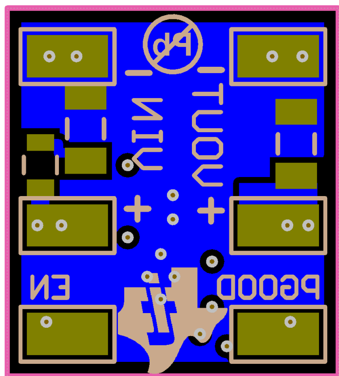
Figure 32. Bottom Copper (Bottom View)
