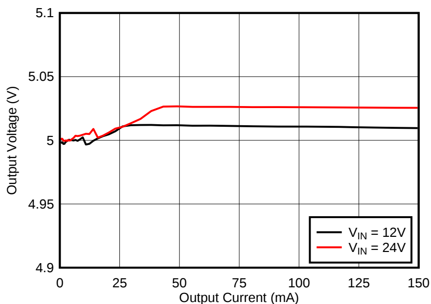
Figure 5. Load Regulation
