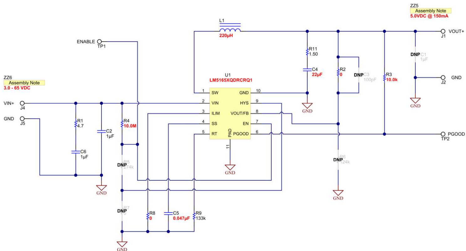
Figure 28. 5V, 150mA COT Schematic (Fixed 5V Output Version)
