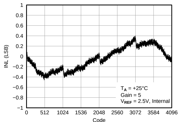
Figure 13. LINEARITY ERROR vs CODE
