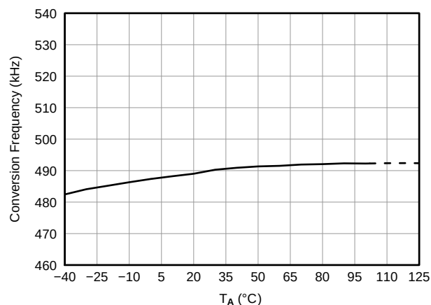
Figure 64. CONVERSION FREQUENCY vs TEMPERATURE
