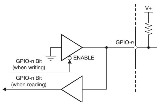
Figure 99. GPIO Pins
