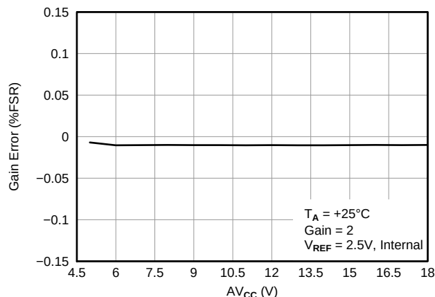
Figure 24. GAIN ERROR vs SUPPLY
