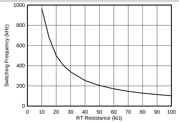
Figure 18. Oscillator Frequency vs RT Resistance
