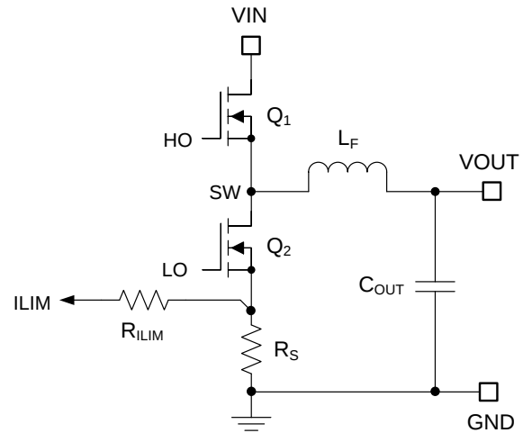
Figure 37. Shunt Resistor Current Sensing
