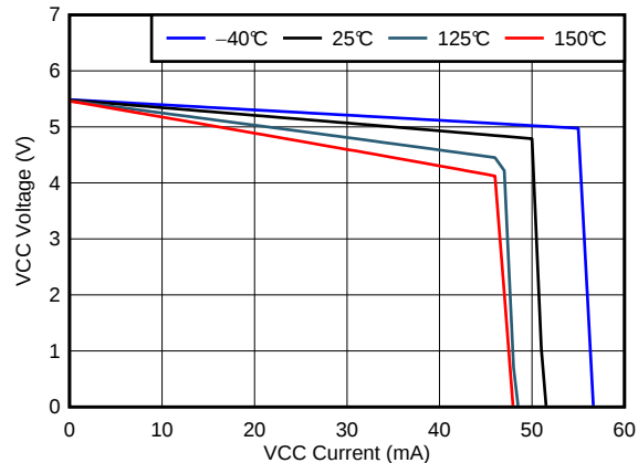
Figure 25. VCC vs ICC Characteristic
