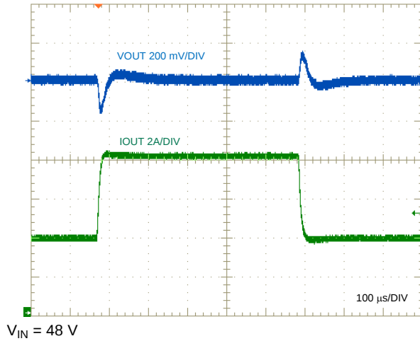
Figure 64. Load Transient Response, 4 A to 8 A to 4 A
