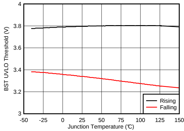
Figure 13. BST UVLO Thresholds vs Junction Temperature
