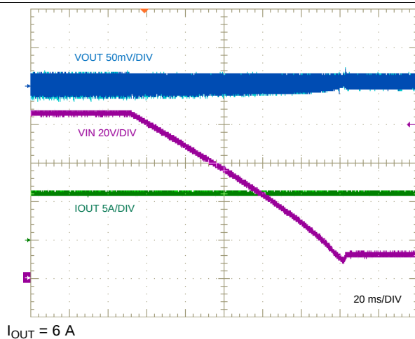
Figure 53. Line Transient Response, 85 V to 12 V
