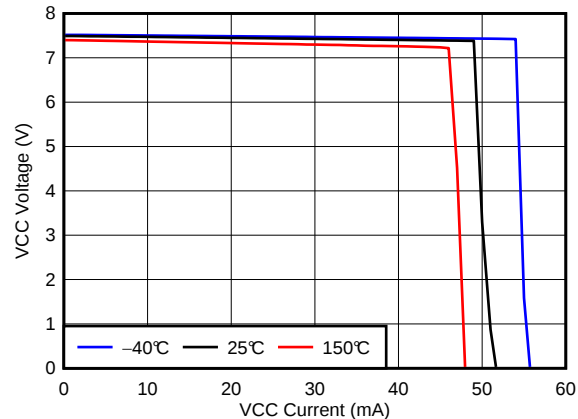
Figure 26. VCC vs ICC Characteristic
