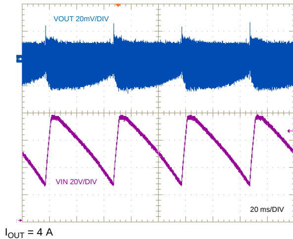
Figure 66. Repetitive Line Transients, 24 V to 75 V
