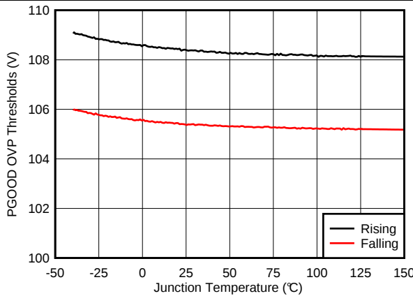
Figure 15. PGOOD OVP Thresholds vs Junction Temperature
