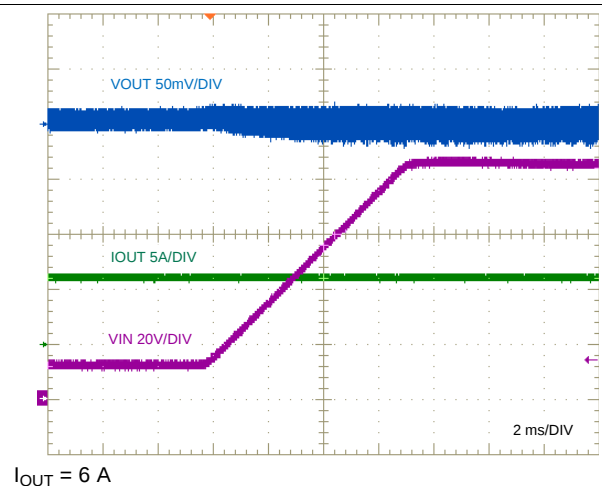
Figure 52. Line Transient Response, 12 V to 85 V
