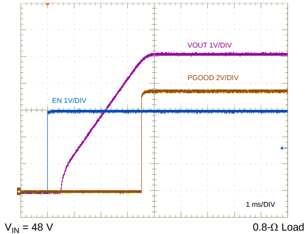
Figure 49. ENABLE ON, Resistive Load
