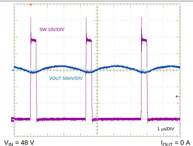
Figure 54. SW Node and Output Ripple Voltages
