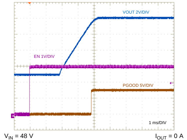
Figure 67. Pre-Biased Start-Up
