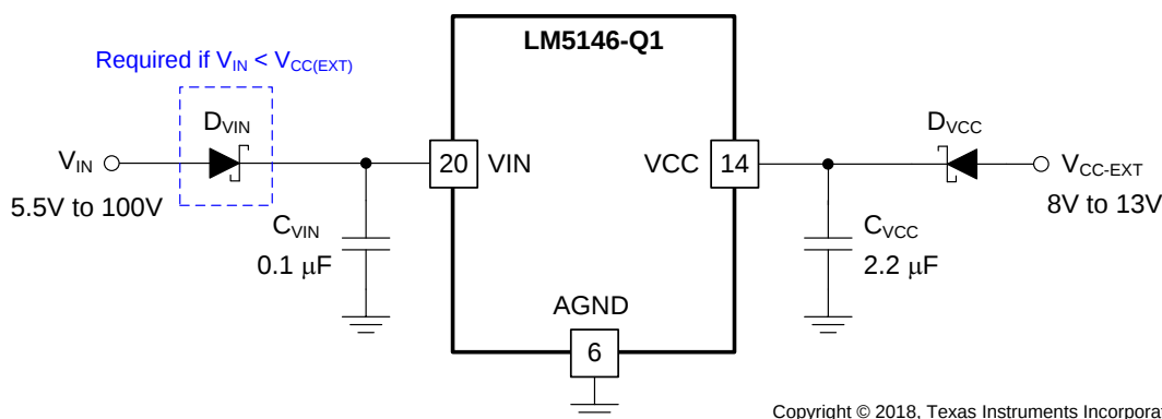
Figure 30. VCC Bias Supply Connection From VOUT or Auxiliary Supply
