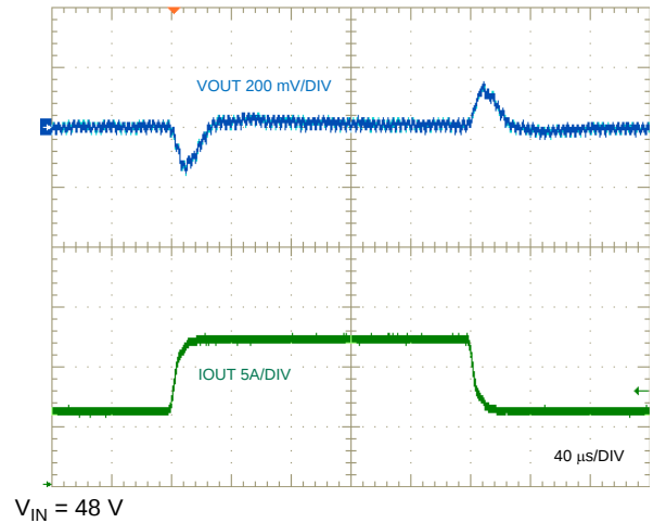
Figure 50. Load Transient Response, 6 A to 12 A to 6 A
