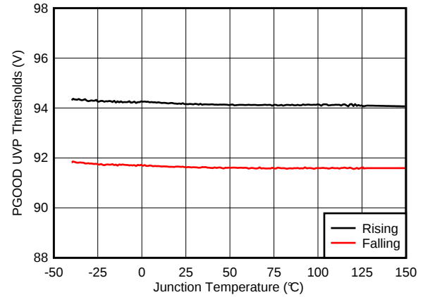
Figure 14. PGOOD UVP Thresholds vs Junction Temperature
