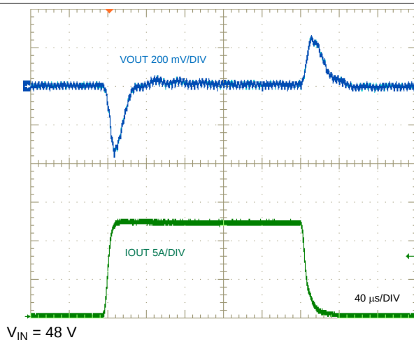
Figure 51. Load Transient Response, 0 A to 12 A to 0 A
