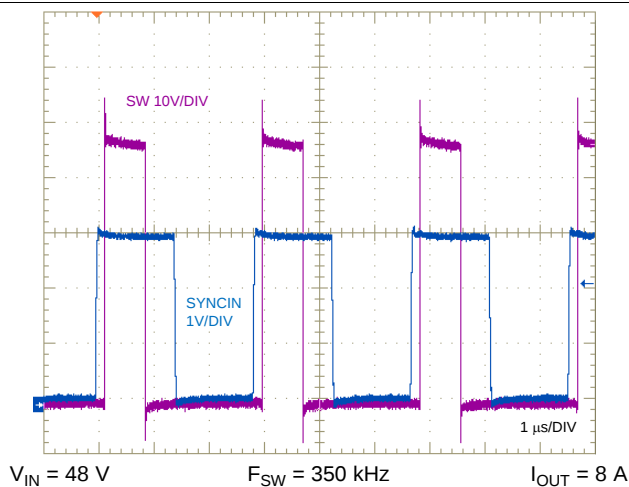
Figure 68. SW Node and SYNCIN Voltages
