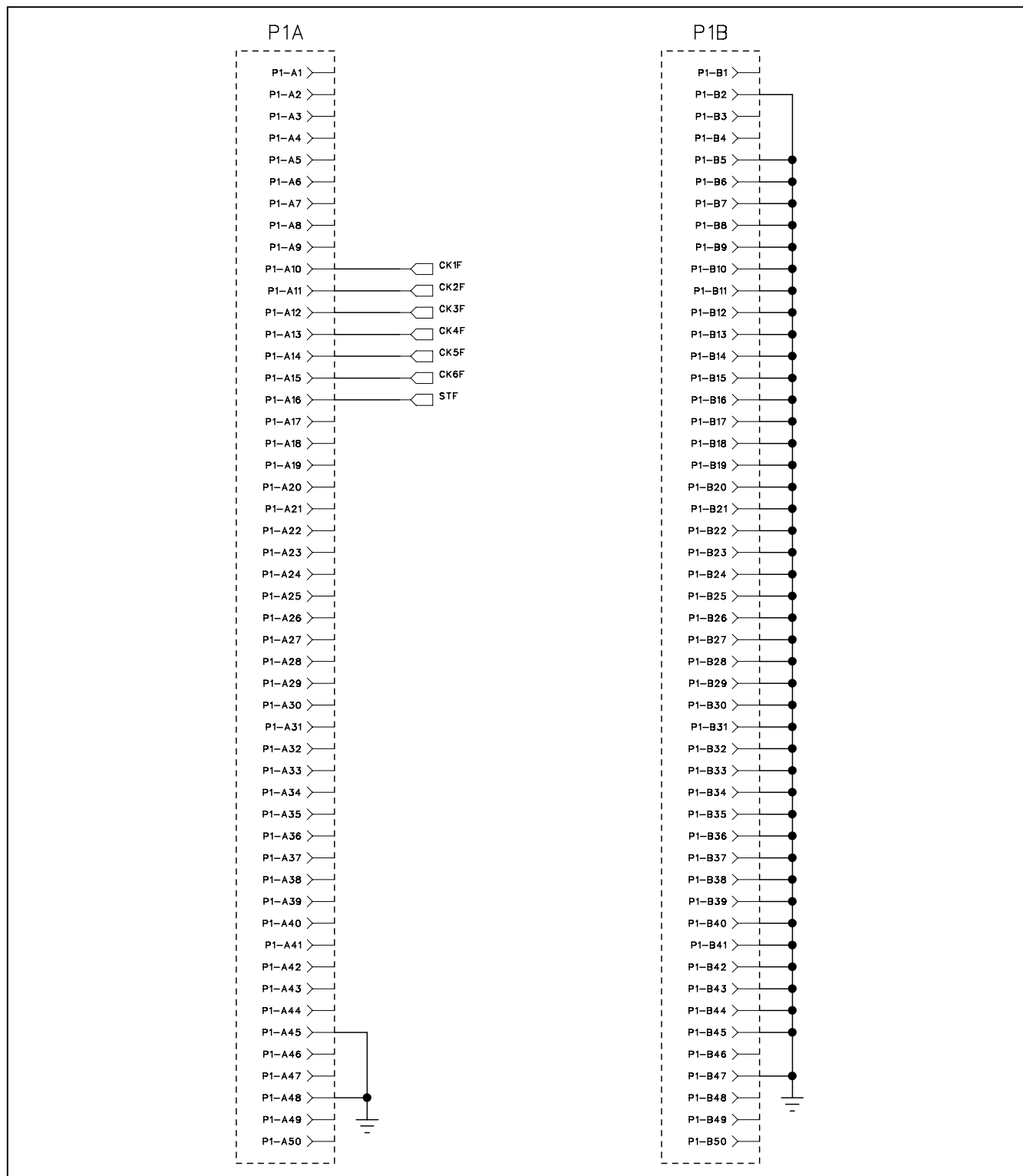
Figure 1c. MAX17117 EV Kit Schematic (Sheet 3 of 3)
