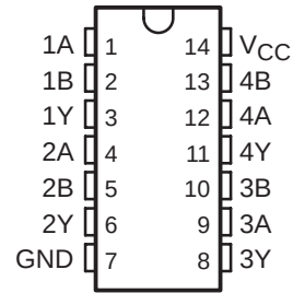
SN54ALS86, SN54AS86A . . . J PACKAGE SN74ALS86, SN74AS86A . . . D OR N PACKAGE (TOP VIEW)
