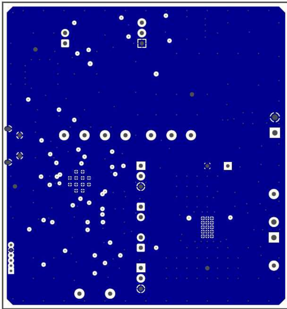
Figure 12. Signal Layer 1
