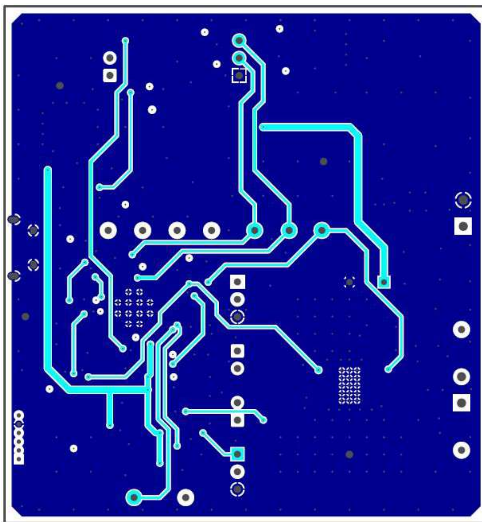
Figure 13. Signal Layer 2
