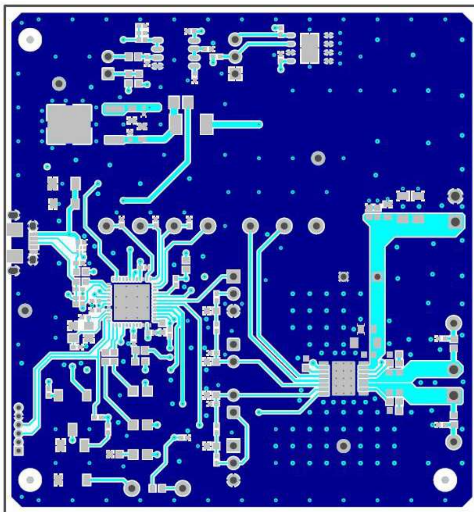
Figure 11. Top Layer
