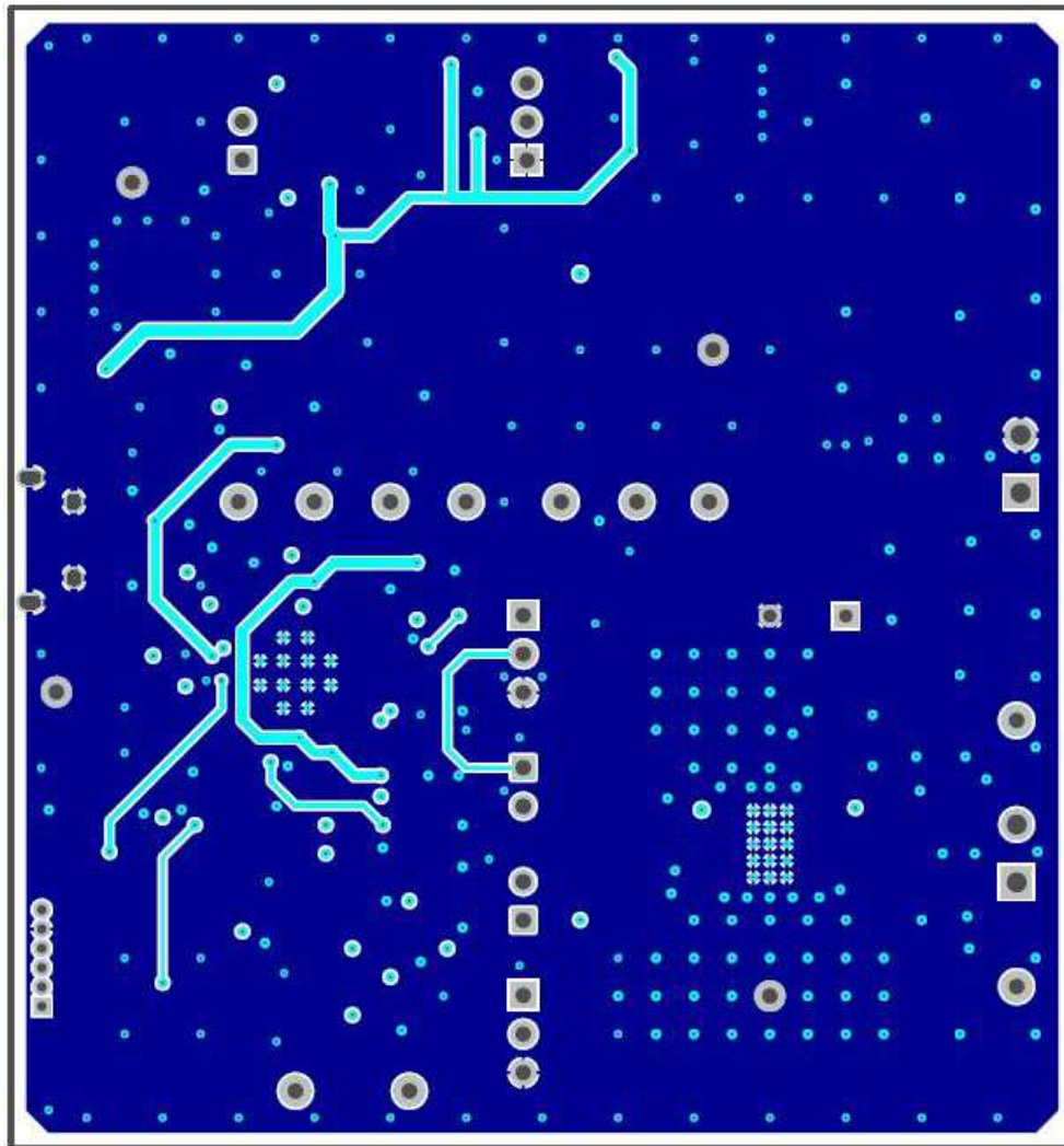
Figure 14. Bottom Layer
