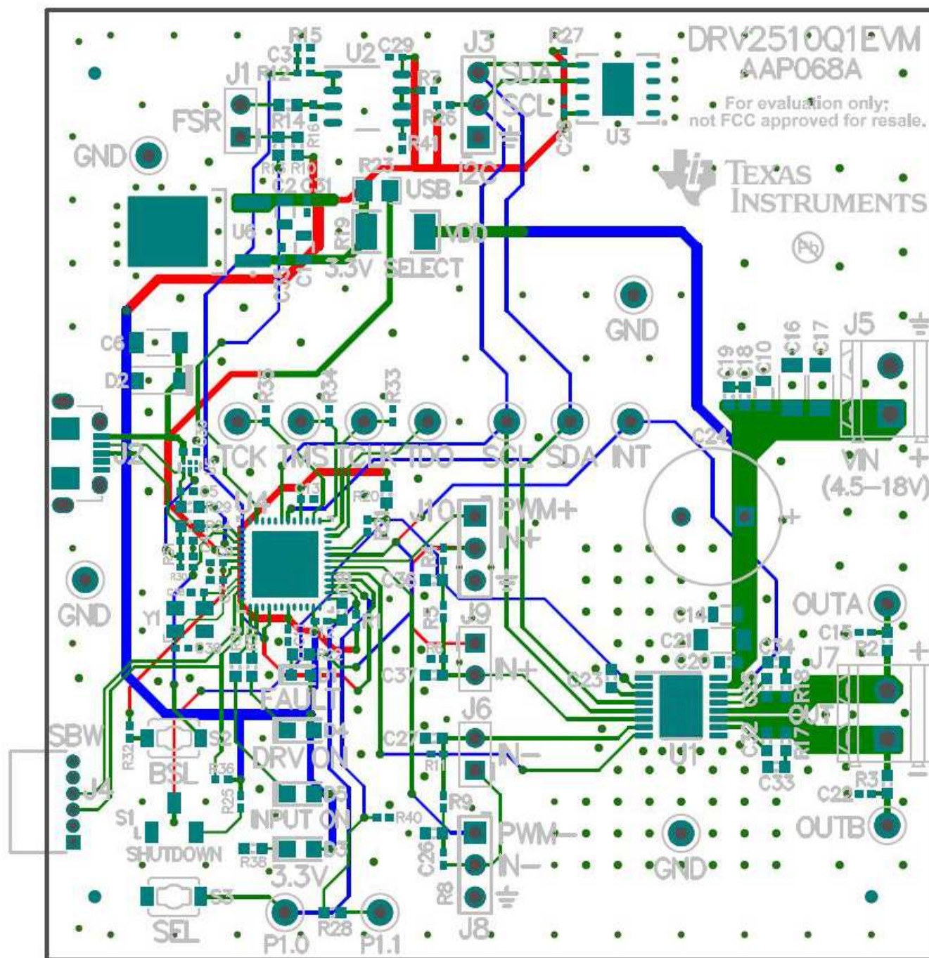
Figure 10. All Layers
