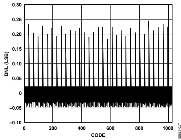
Figure 17. Typical DNL
