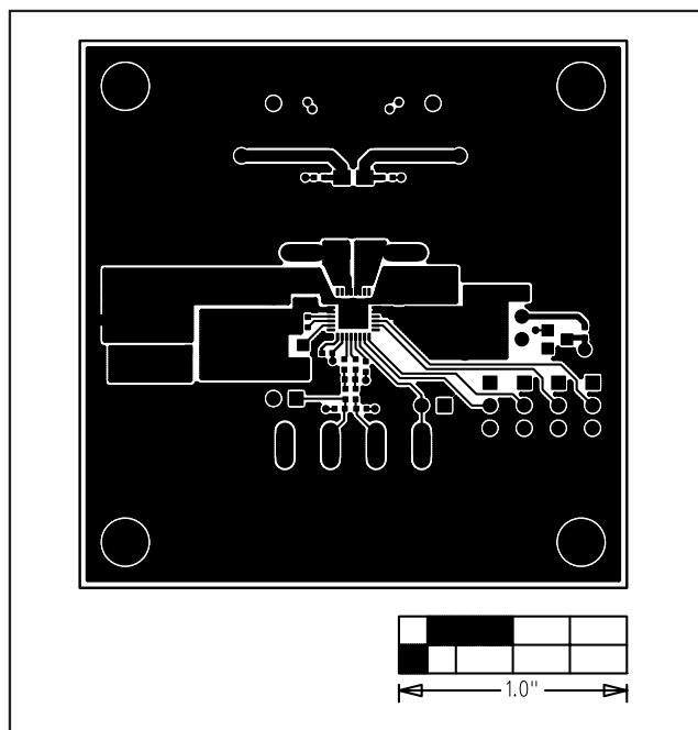
Figure 3. MAX9713 EV Kit PCB—Component Side
