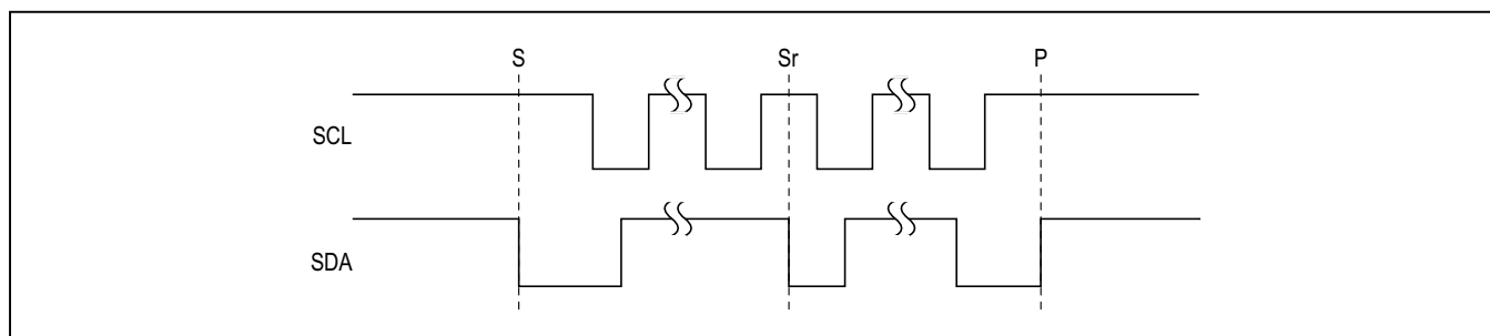
Figure 21. START, STOP, and REPEATED START Conditions
