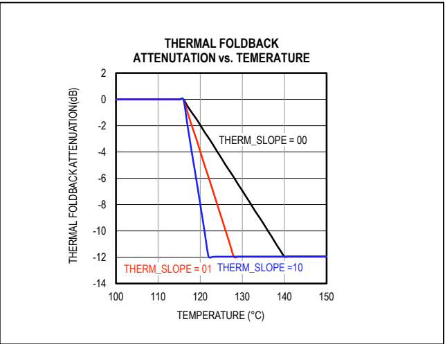
Figure 15. Thermal Foldback Performance
