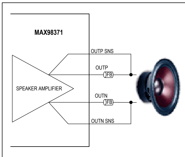
Figure 19. Typical Application Circuit with Ferrite Beads Used
