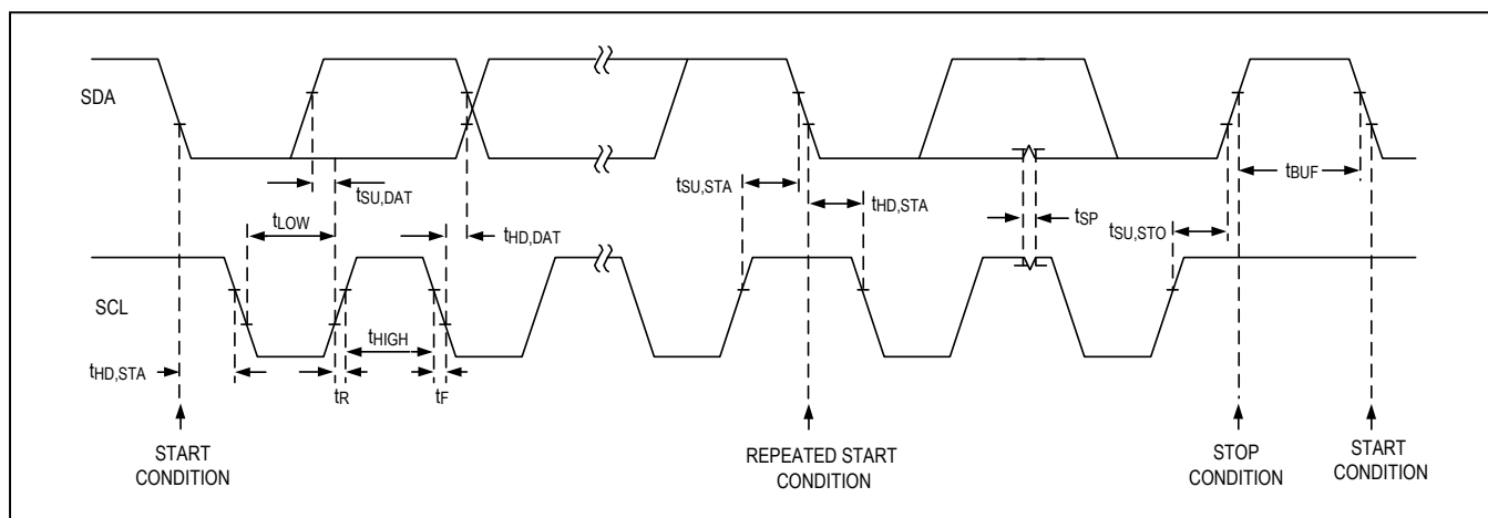
Figure 4. I 2 C Interface Timing Diagram
