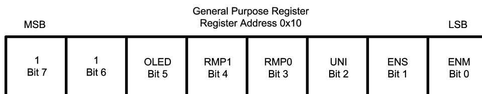
Figure 7. General Purpose Register Description
