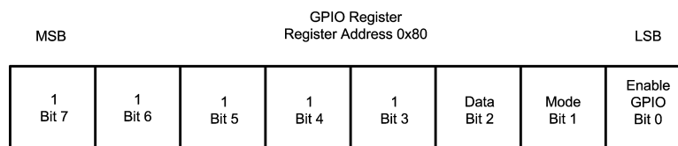
Figure 11. GPIO Register Description
