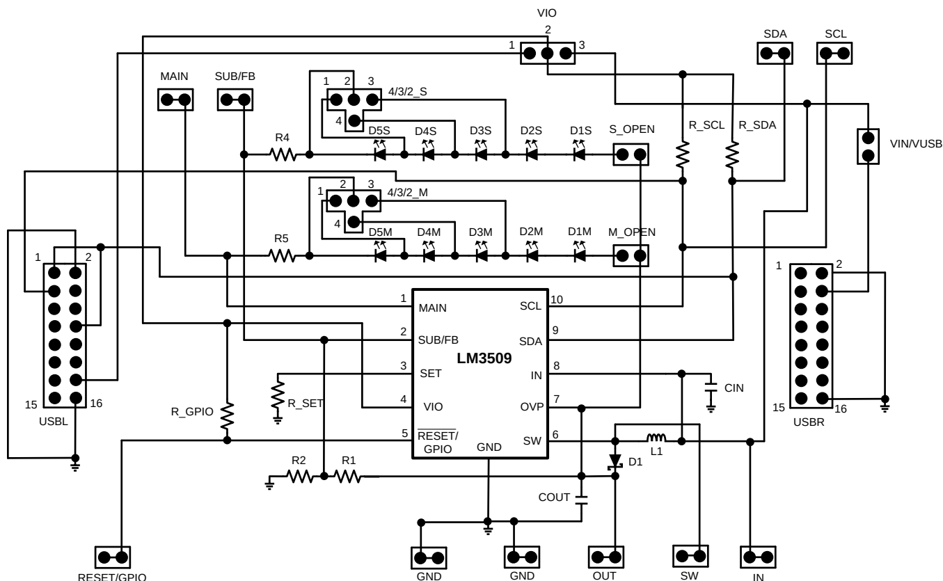
Figure 1. LM3509 Evaluation Board Schematic
