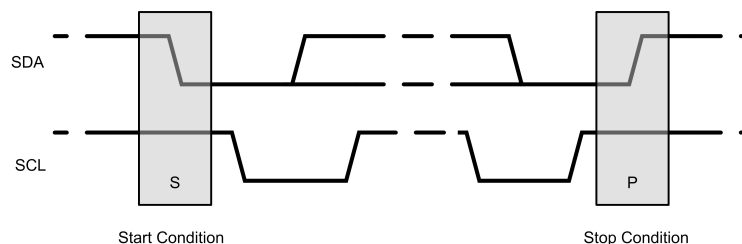
Figure 4. Start and Stop Sequences
