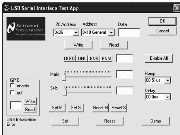
Figure 12. LM3509.exe
