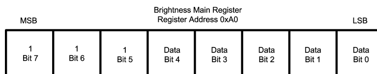
Figure 8. Brightness MAIN Register Description
