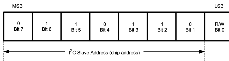
Figure 5. Chip Address
