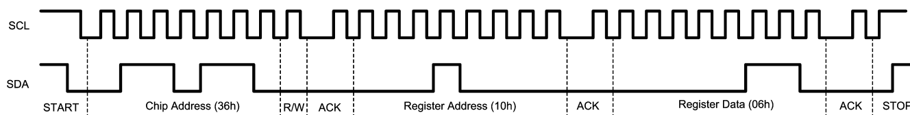
Figure 6. Write Sequence to the LM3509
