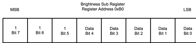
Figure 9. Brightness SUB Register Description
