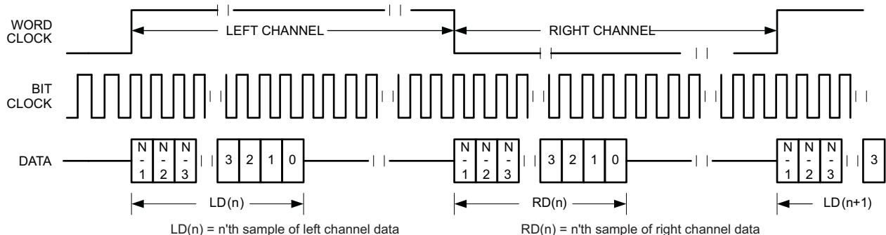
Figure 44. Timing Diagram for Left-Justified Mode with ASI_OFFSET1 = 0 and Inverted Bit Clock
