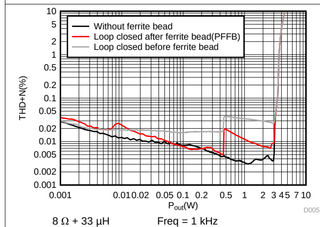
Figure 11. THD+N vs Output Power
