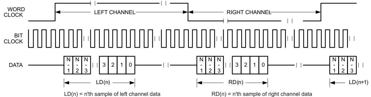
Figure 43. Timing Diagram for Left-Justified Mode with ASI_OFFSET1 = 1
