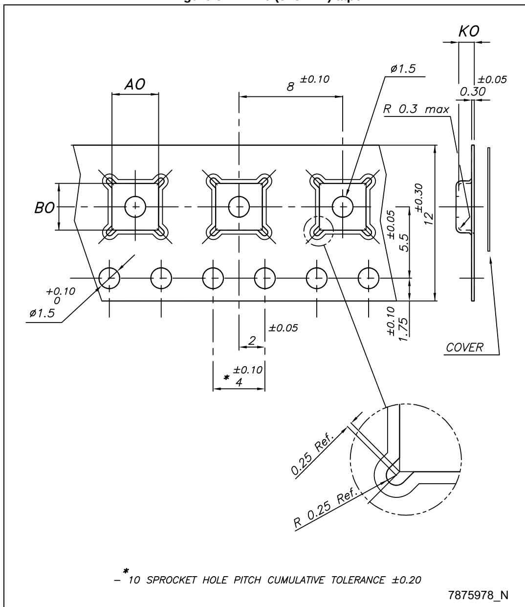
Figure 32. DFN6 (3x3 mm) tape
