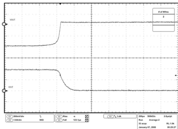
Figure 23. Enable transient
