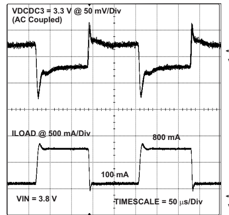
Figure 18. VDCDC3 Load Transient Response
