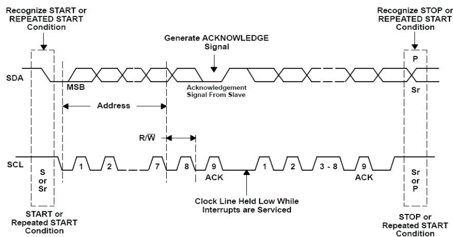
Figure 57. Bus Protocol
