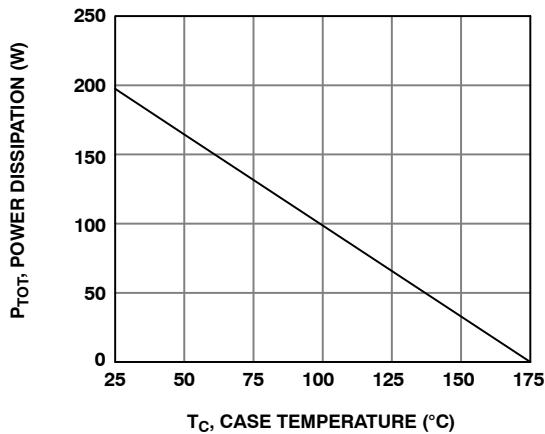
Figure 4. Power Dissipation
