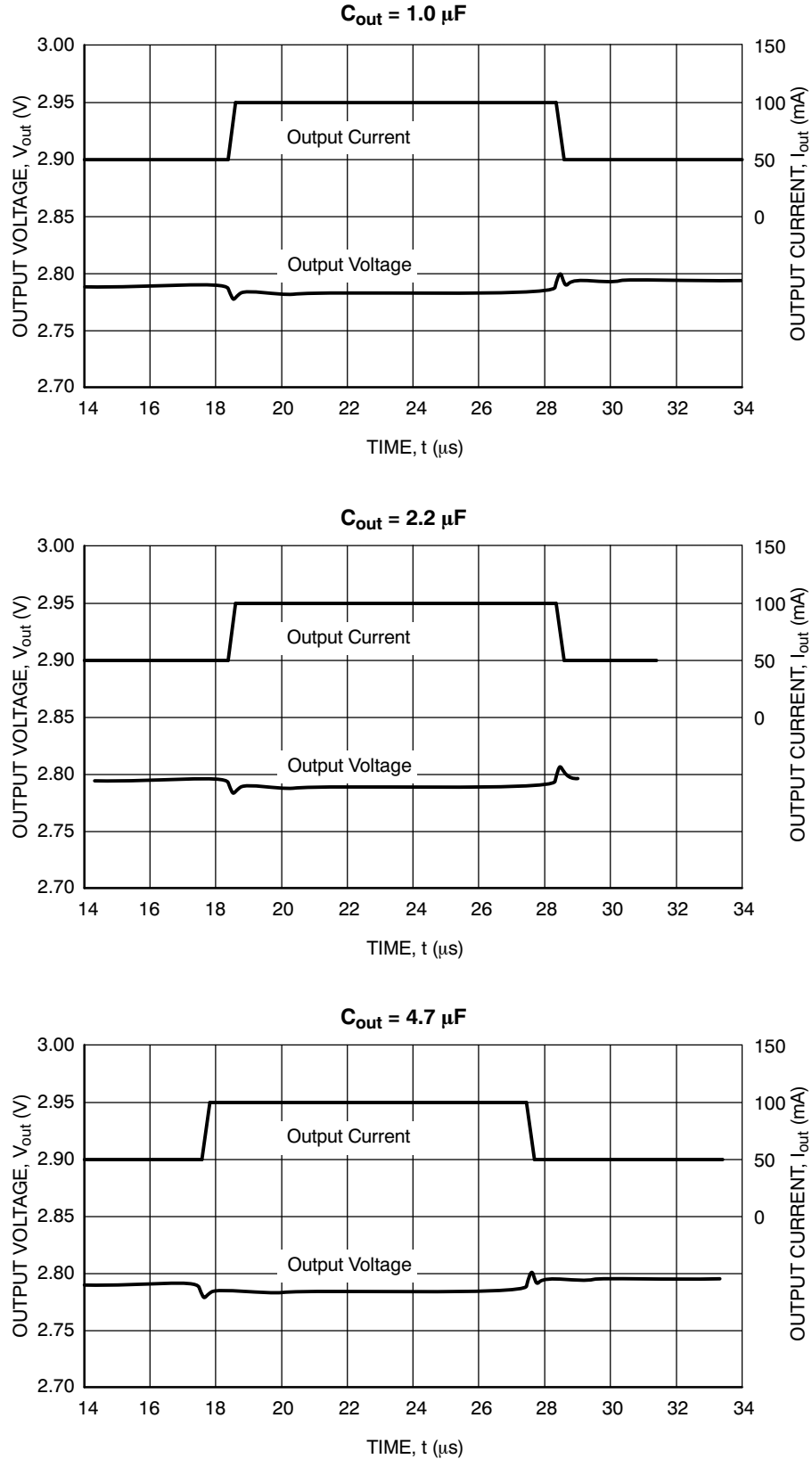
Figure 17. Load Transient Response (V_{in} = 3.8 V, I_{out} = 50 mA \text{ to } 100 mA, tr = tf = 5.0 \mu s, C_{in} = 1.0 \mu F, V_{out} = 2.8 V)
