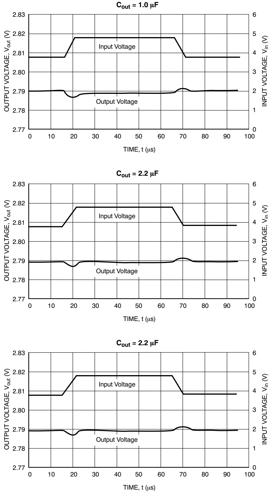
Figure 16. Input Transient Response ( V_{in} = 3.8 \text{ V to } 4.8 \text{ V} , I_{out} = 30 \text{ mA} , t_r = t_f = 5.0 \mu s , V_{out} = 2.8 \text{ V} )
