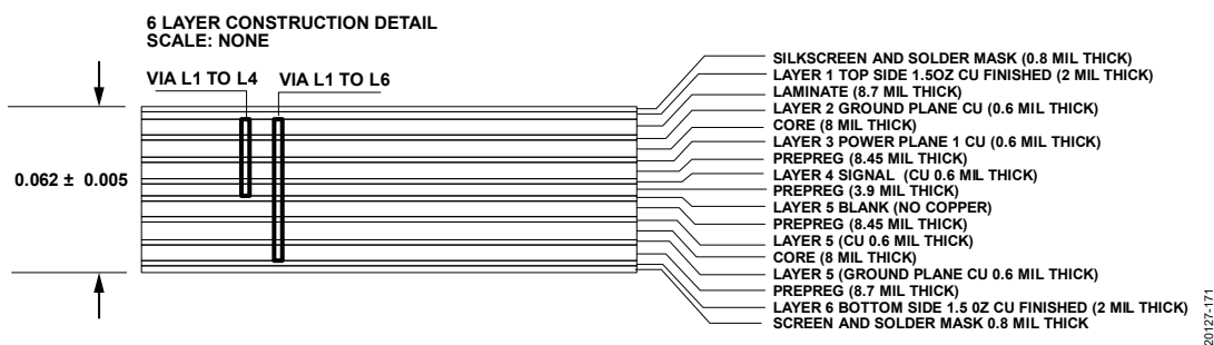
Figure 71. PCB Stackup
