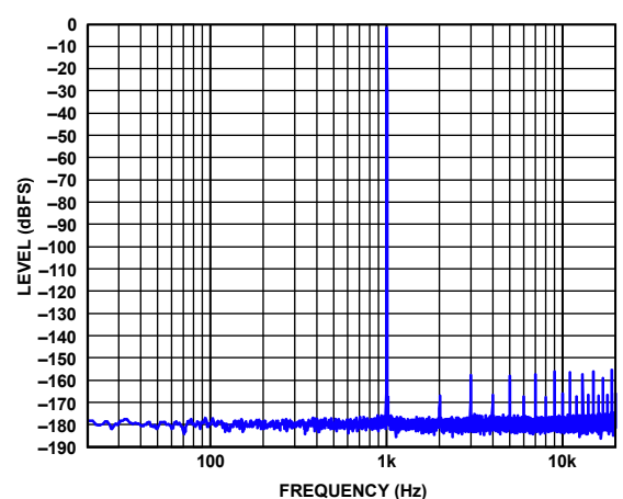
Figure 39. FFT, -1 dBFS, f_s = 48 kHz Throughout Except FastDSP = 768 kHz, Signal Path = SDATAI_x to SigmaDSP to Interpolator to FastDSP to Decimator to SDATAO_x
