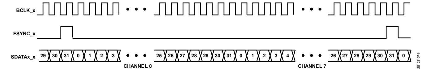
Figure 69. 8-Channel TDM Mode, Default Settings, Except SPTx_SAI_MODE = 1
