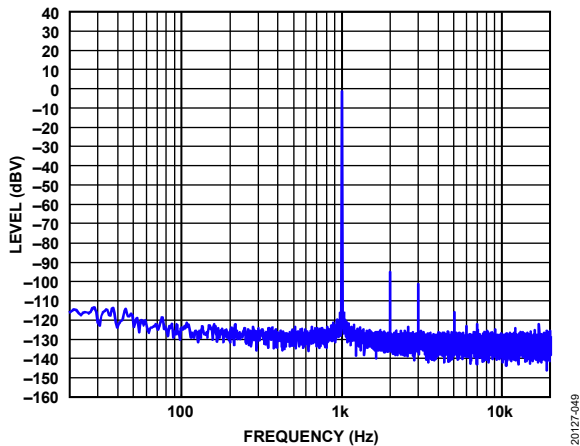
Figure 48. FFT, -1 dBV, Line Output Mode, Load = 10\ \text{k}\Omega , f_s = 48\ \text{kHz} to 768\ \text{kHz} , Signal Path = AIN0 to LOUTLx
