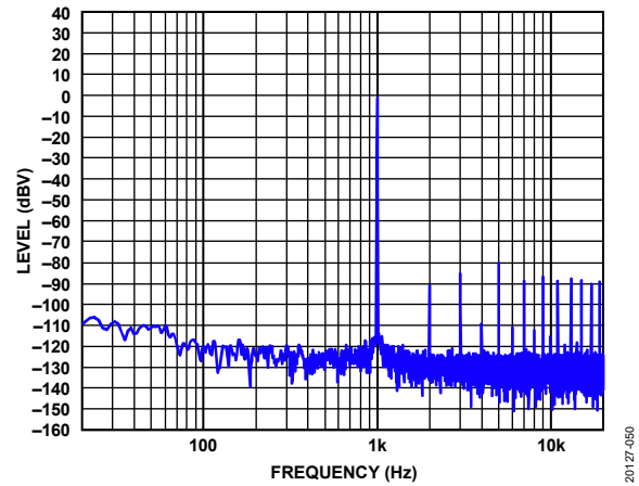
Figure 49. FFT, -1 dBV, Headphone Mode, Load = 16\ \Omega , f_s = 48\ \text{kHz} to 768\ \text{kHz} , Signal Path = AINx to HPOUTxx
