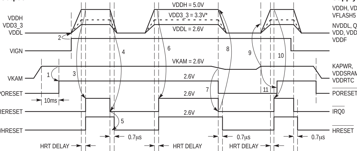
Figure 5. 33394 Timing Diagram
