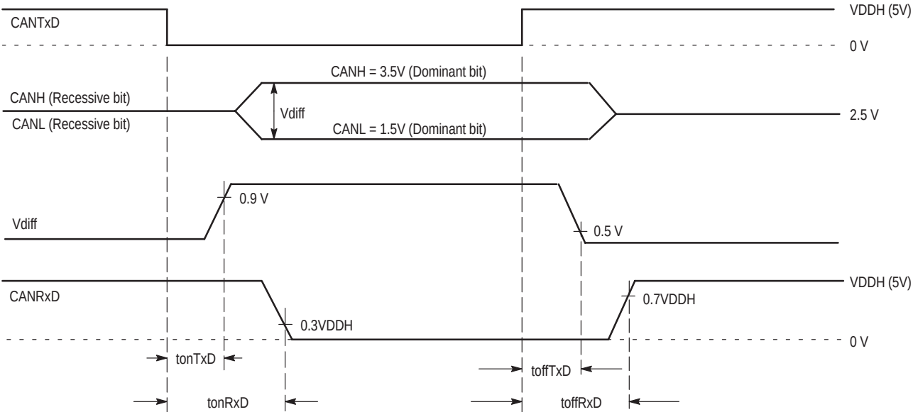
Figure 2. CAN Delay Timing Waveform
