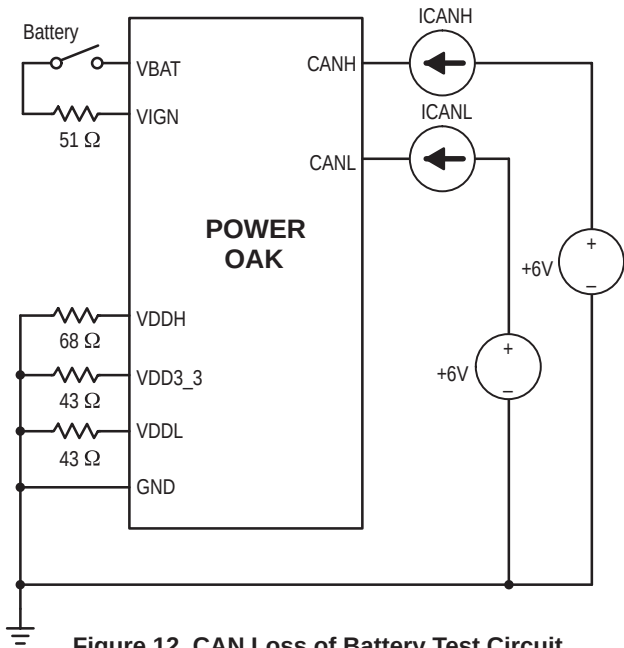
Figure 12. CAN Loss of Battery Test Circuit
