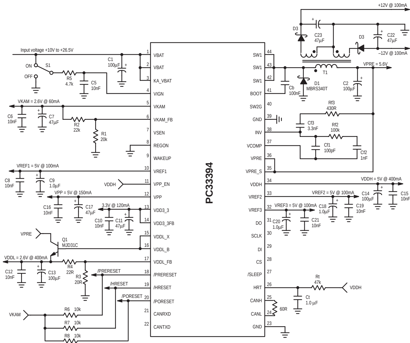
Figure 23. 33394 Flyback Converter Provides Symmetrical Voltages
