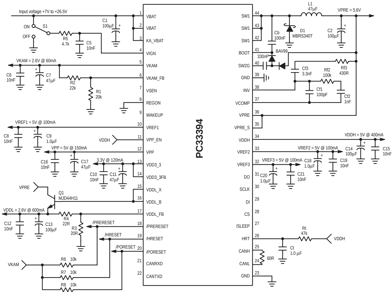
Figure 22. 33394 Buck-Only Application
