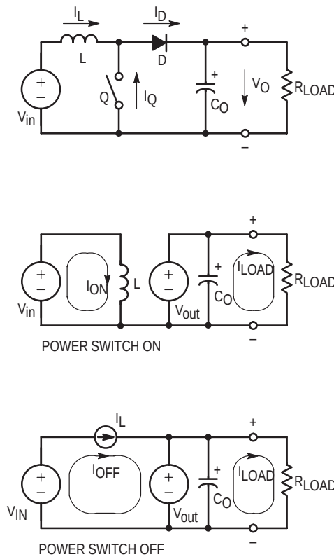
Figure 14. Basic Boost Converter Operation and its Waveforms
