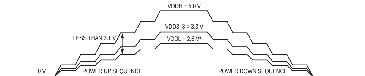
Figure 6. 33394 Power Up/Down Sequence
