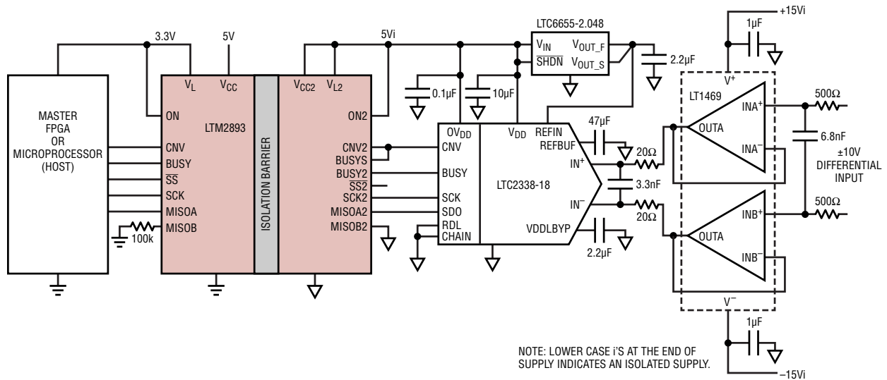
Figure 13. Isolated 1MSPS LTC2338-18 Fully Differential \pm 10\text{V} Input Range, with ADC Sleep Disabled (CNV2 = BUSYS)
