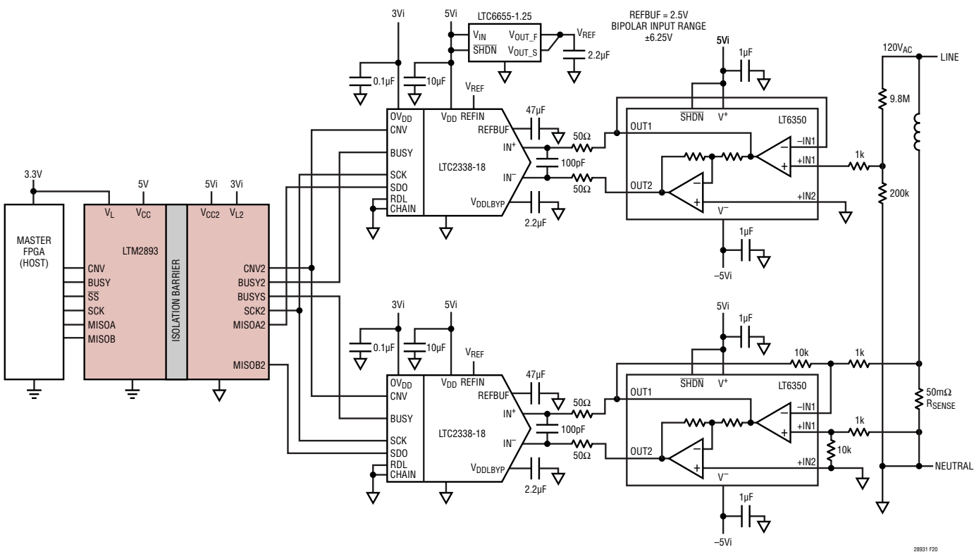
Figure 20. Simultaneous Sampled Line Current and Voltage Measurements with Two LTC2338-18 ADCs
