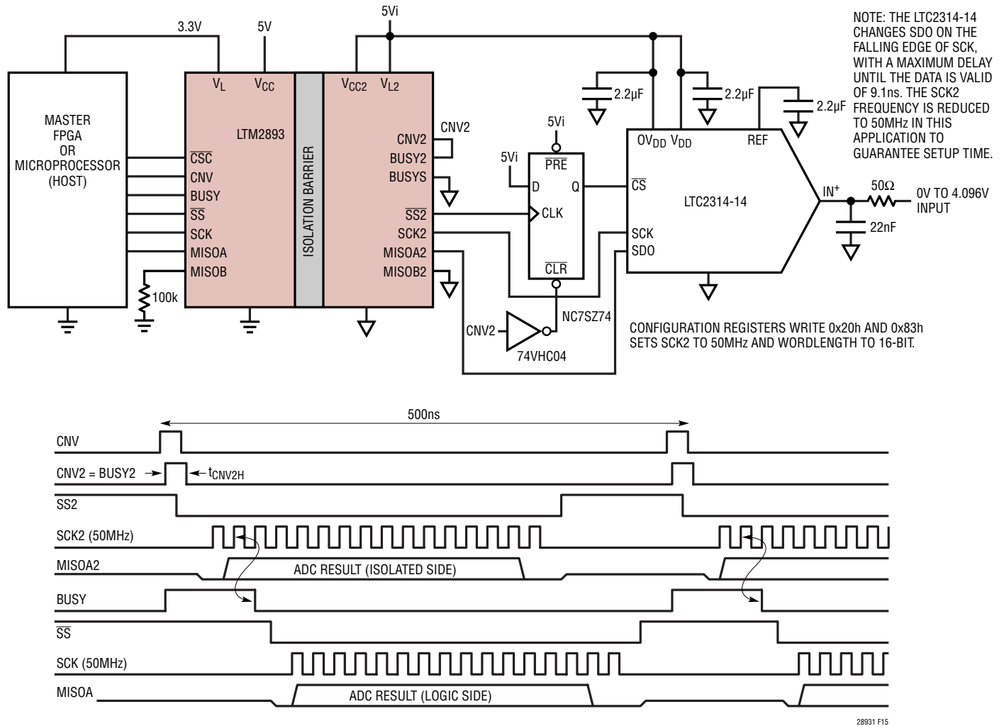
Figure 15. Isolated 2Msps LTC2314-14 0V to 4.096V Input Range, ADC Without a CNV or BUSY, LTC2314 \overline{CS} Is Synchronized to Low Jitter CNV2
