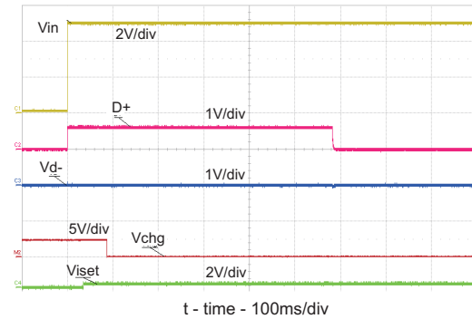
Figure 2. D+ D- Detection for Unknown Source Hot Plug
