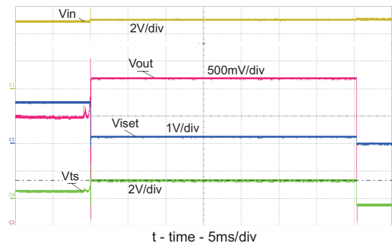
Figure 7. Battery Removal – GND Removed First
