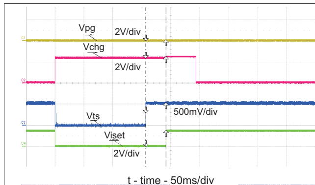
Figure 26. TS Enable and Disable
