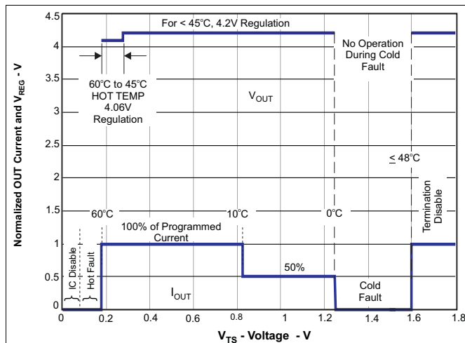
Figure 22. Operation Over TS Bias Voltage
