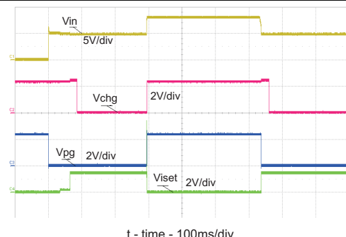
Figure 6. OVP from Normal Operation
