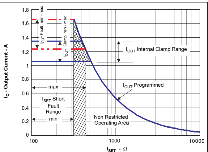
Figure 23. Programmed / Clamped Out Current
