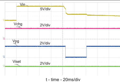
Figure 5. OVP 8-V Adaptor – Hot Plug
