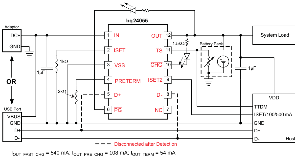
Figure 28. Typical Application Circuit, bq24055
