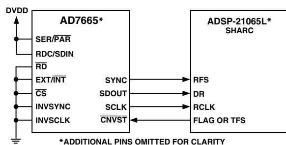
Figure 23. Interfacing to the ADSP-21065L Using the Serial Master Mode
