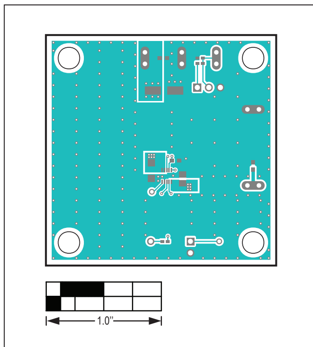
MAXM15065 EV Kit PCB Layout—Top Layer
