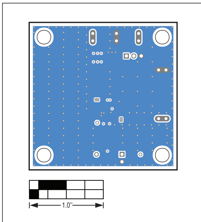
MAXM15065 EV Kit PCB Layout—Bottom Layer
