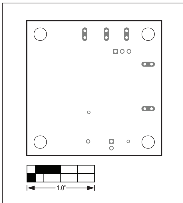
MAXM15065 EV Kit PCB Layout—Silk Bottom
