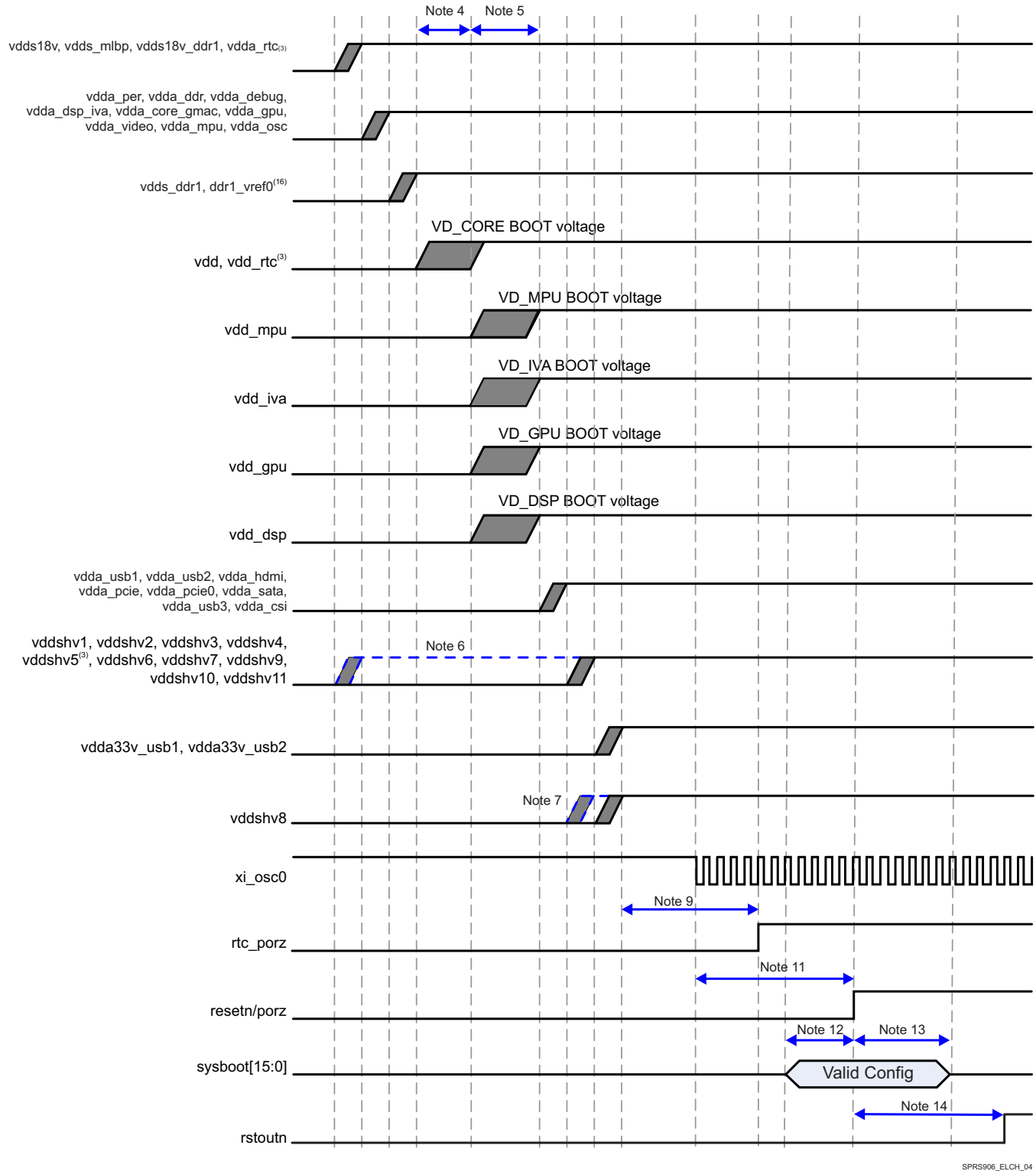
Figure 5-2. Power-Up Sequencing
