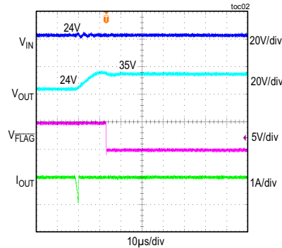
REVERSE-BLOCKING RESPONSE
