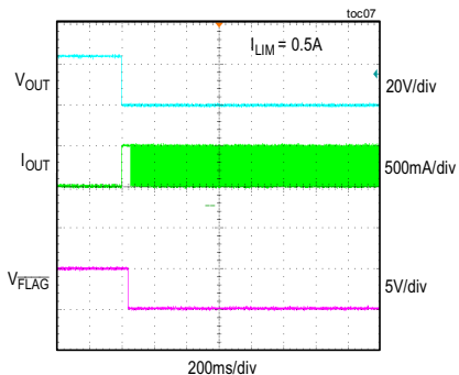
CONTINUOUS CURRENT-LIMIT RESPONSE
