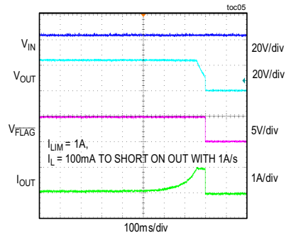
CURRENT-LIMIT RESPONSE
