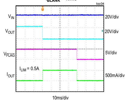
OUTPUT SHORT-CIRCUIT RESPONSE t BLANK = 40ms
