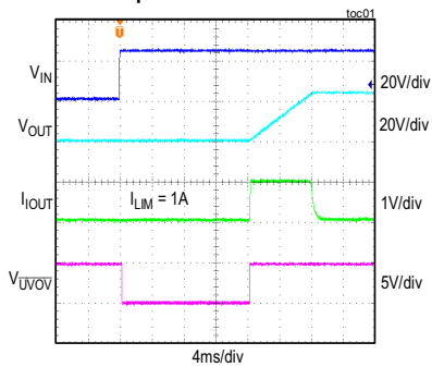
POWER-UP RESPONSE WITH 330 \mu F CAPACITOR AT NO LOAD
