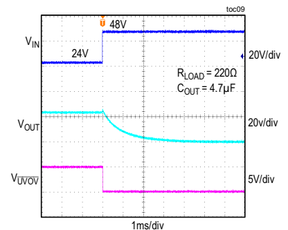
OVERVOLTAGE-FAULT RESPONSE
