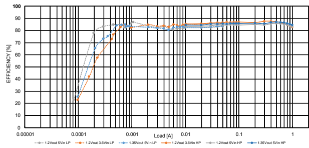
Figure 4. BUCK2 efficiency
