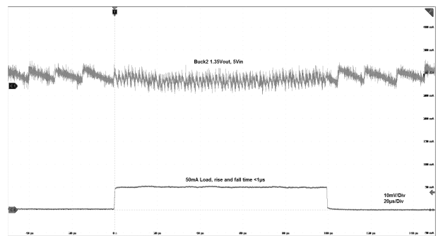
Figure 12. Buck2 load transient in LP mode
