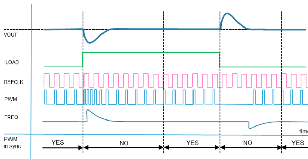
Figure 42. PWM clock generation
