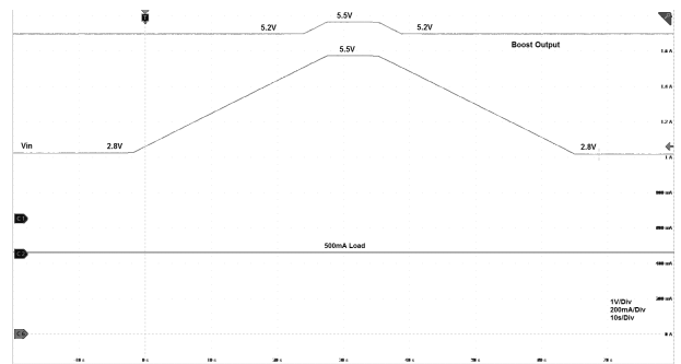
Figure 24. Boost output vs. input voltage
