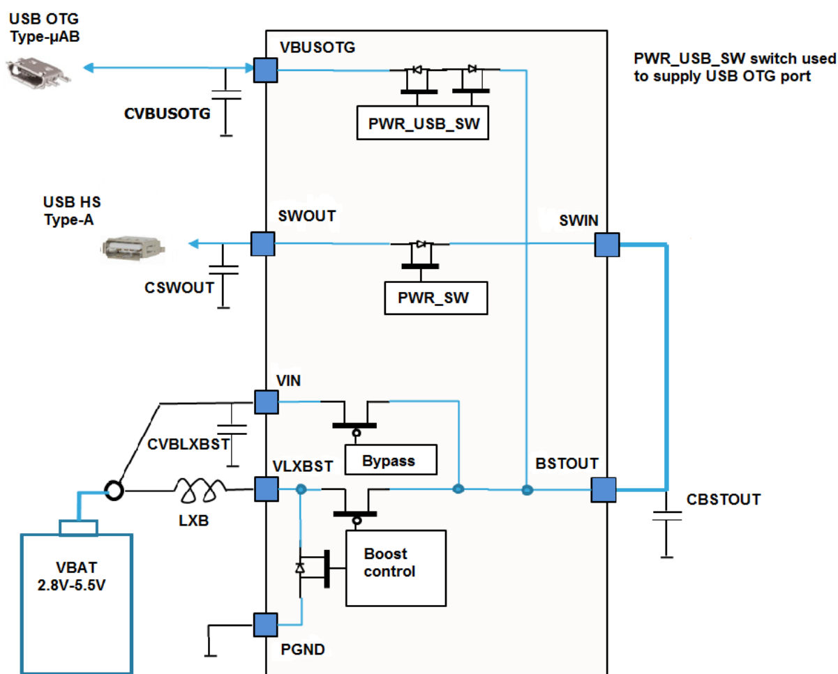
Figure 50. Battery powered application with a USB OTG port and a USB host port
