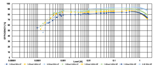
Figure 6. BUCK4 efficiency
