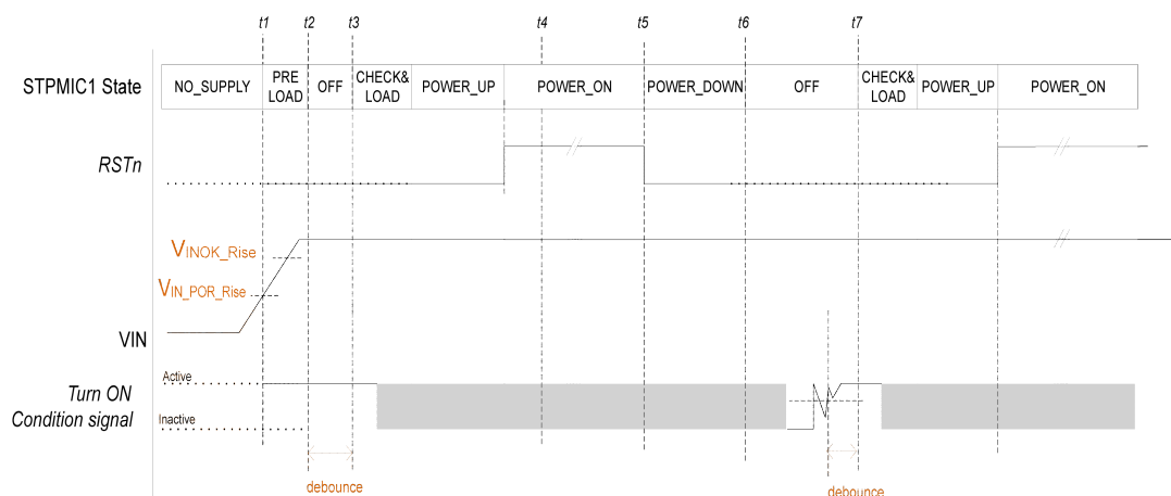
Figure 58. Turn-on condition before V_{IN\_POR\_Rise}
