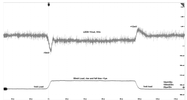
Figure 22. LDO6 load transient
