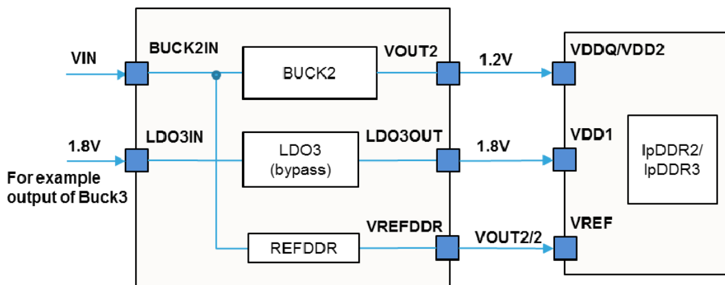
Figure 39. Powering IpDDR2/IpDDR3 memory (LDO3 in bypass mode)
