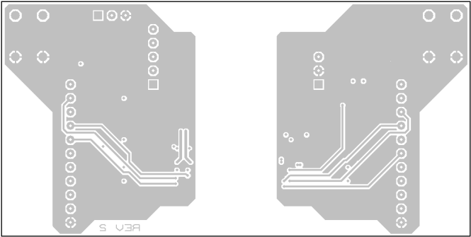
Bottom Copper
