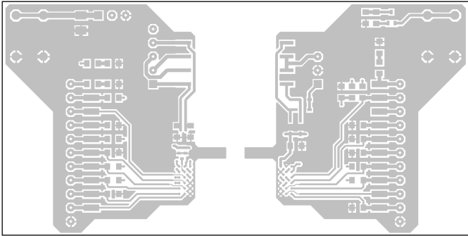
Top Copper
