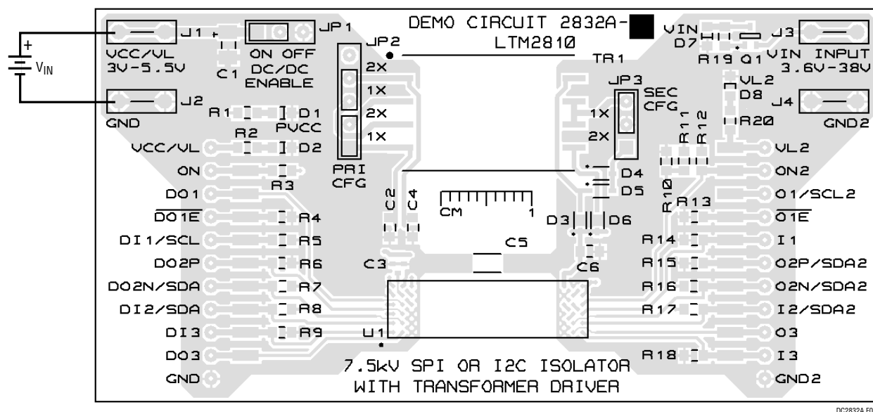
Figure 2. Demo Board Setup
