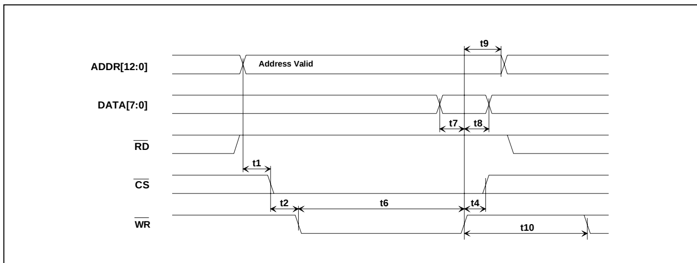
Figure 11-10. Intel Bus Write Timing (HWMODE = 0, MODEC = 00)
