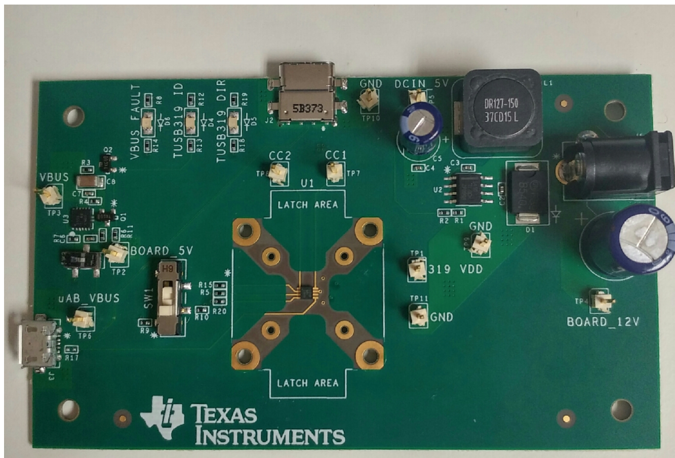
Figure 2. TUSB319EVM
