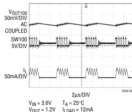
Burst Mode Operation 100mA Channel
