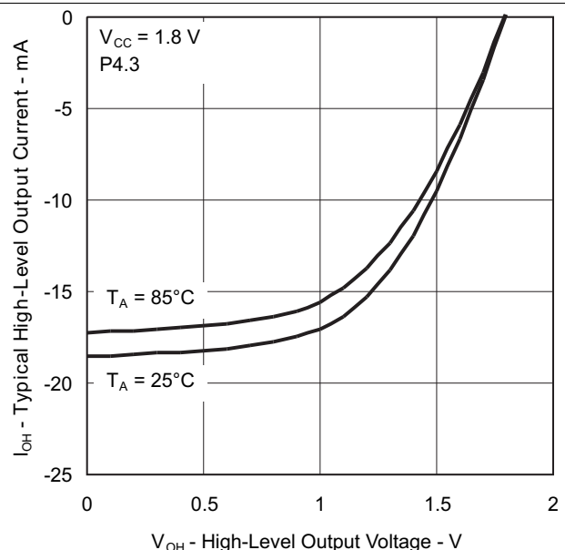
Figure 5-14. Typical High-Level Output Current vs High-Level Output Voltage
