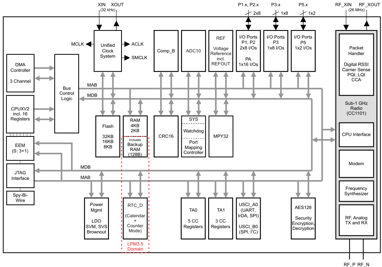
Figure 1-2. CC430F514x Functional Block Diagram
