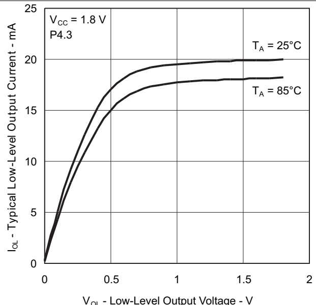
Figure 5-12. Typical Low-Level Output Current vs Low-Level Output Voltage
