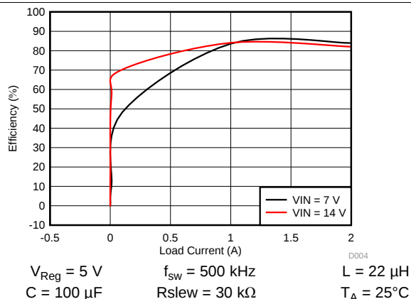
Figure 2. Efficiency vs Load Current for Different Vin
