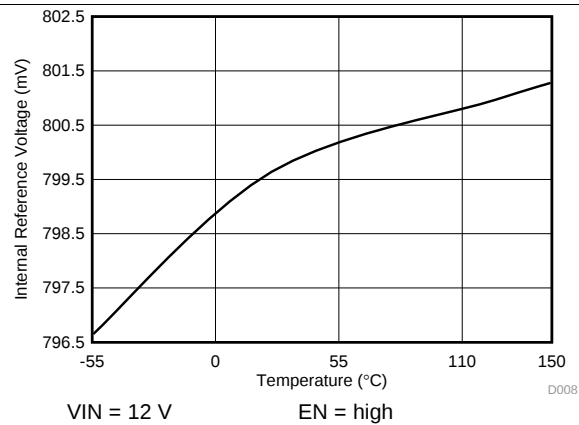
Figure 7. Internal Reference Voltage
