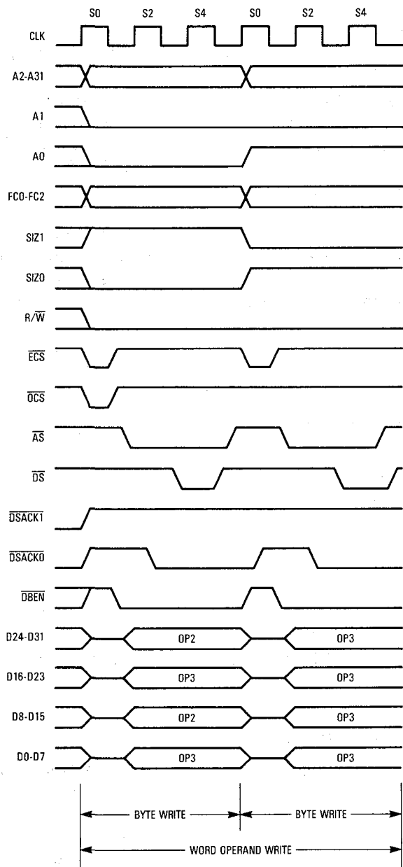
Figure 7-8. Word Operand Write Timing (8-Bit Data Port)
