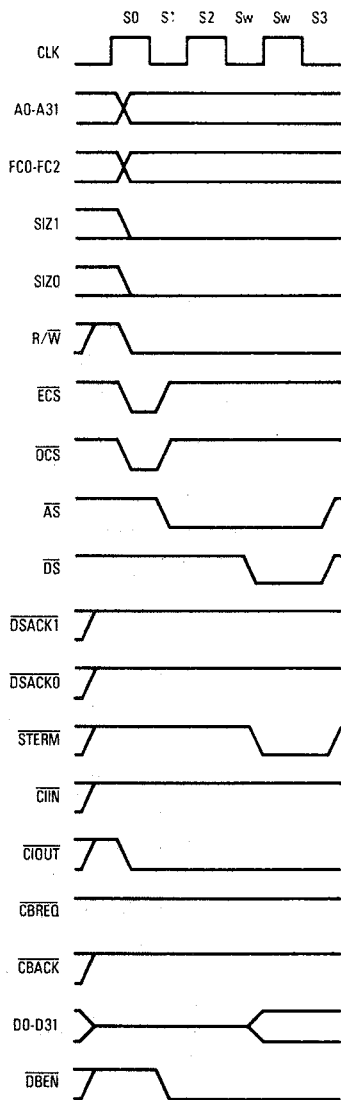
Figure 7-34. Synchronous Write Cycle with Wait States — \overline{\text{CIOUT}} Asserted
