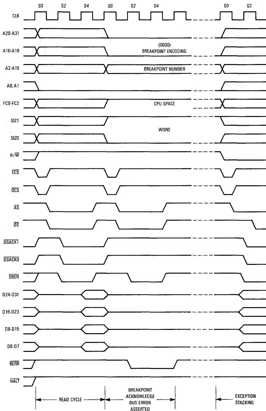
Figure 7-49. Bus Error without \overline{\text{DSACKx}}
