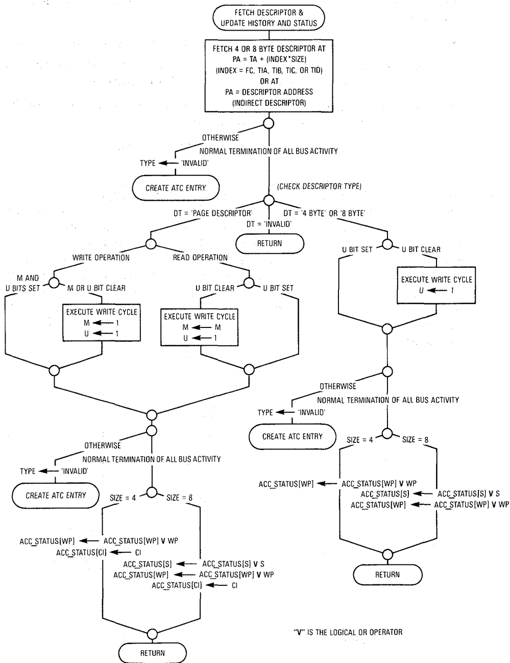
Figure 9-29. Detailed Flowchart of Descriptor Fetch Operation
