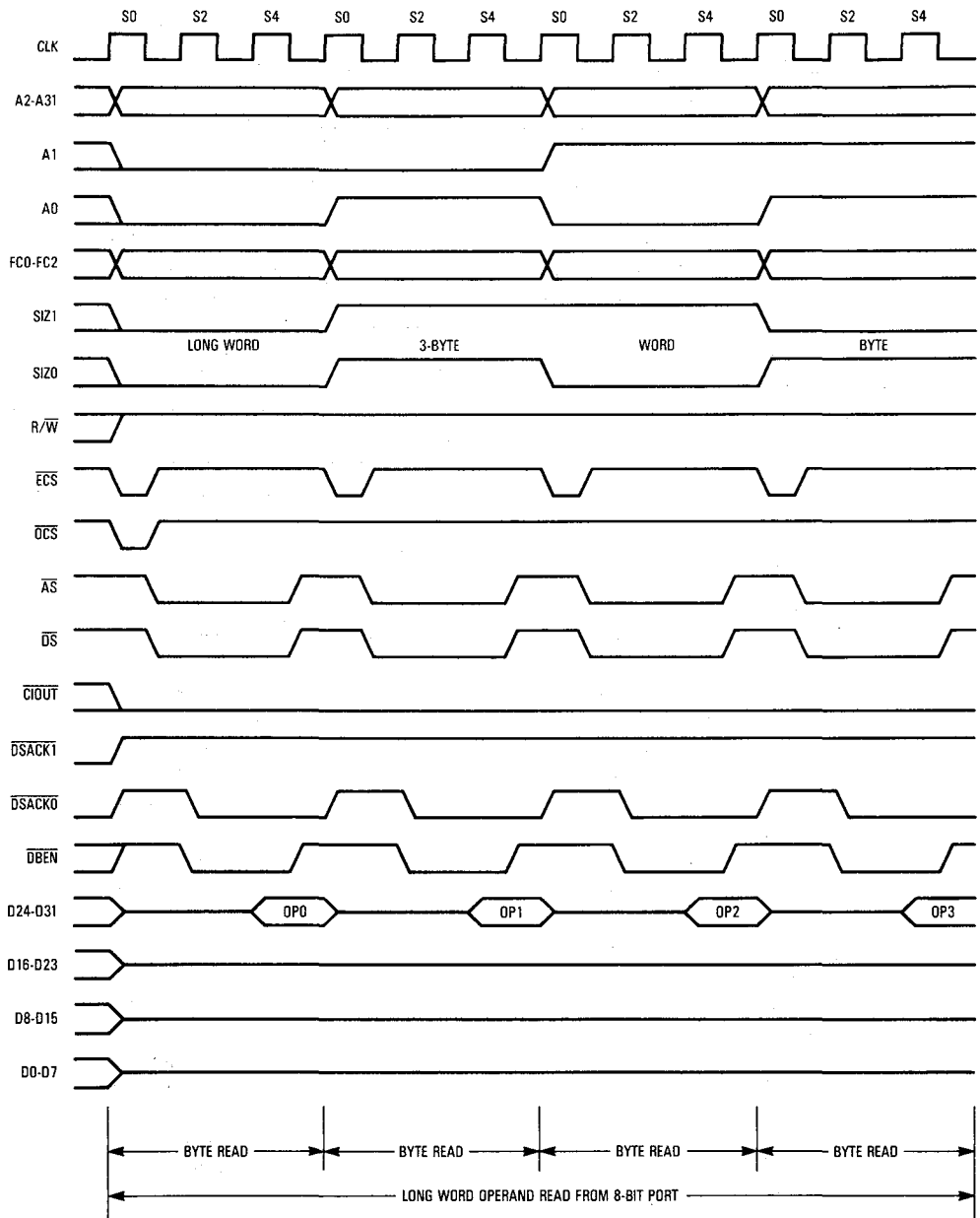
Figure 7-22. Long-Word Read — 8-Bit Port with \overline{\text{CIOOUT}} Asserted
