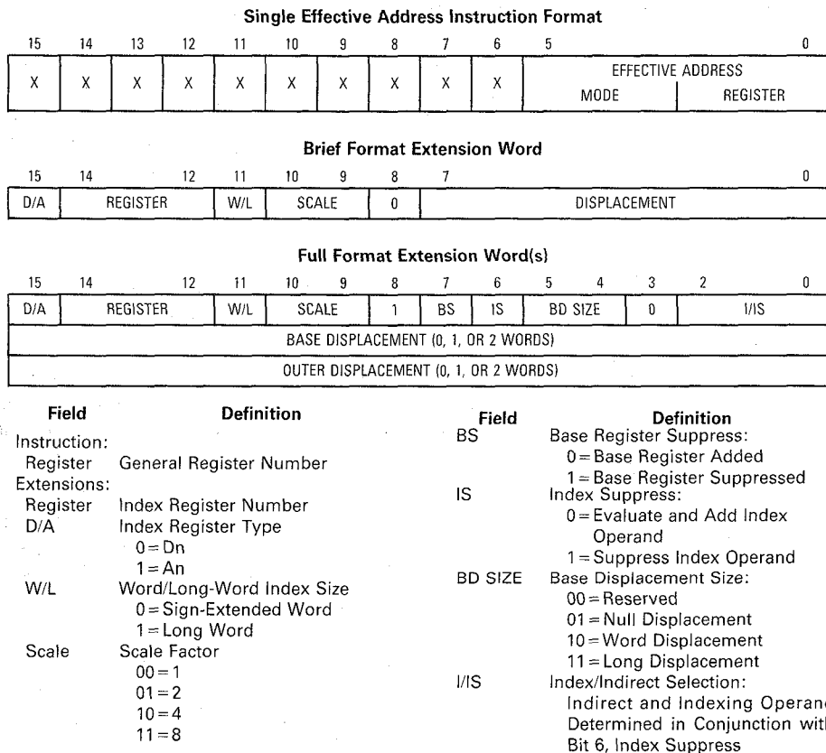
Figure 2-4. Effective Address Specification Formats
