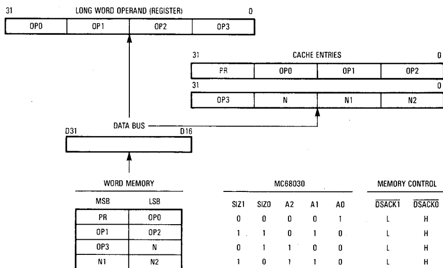
Figure 7-11. Misaligned Cacheable Long-Word Transfer from Word Port Example
