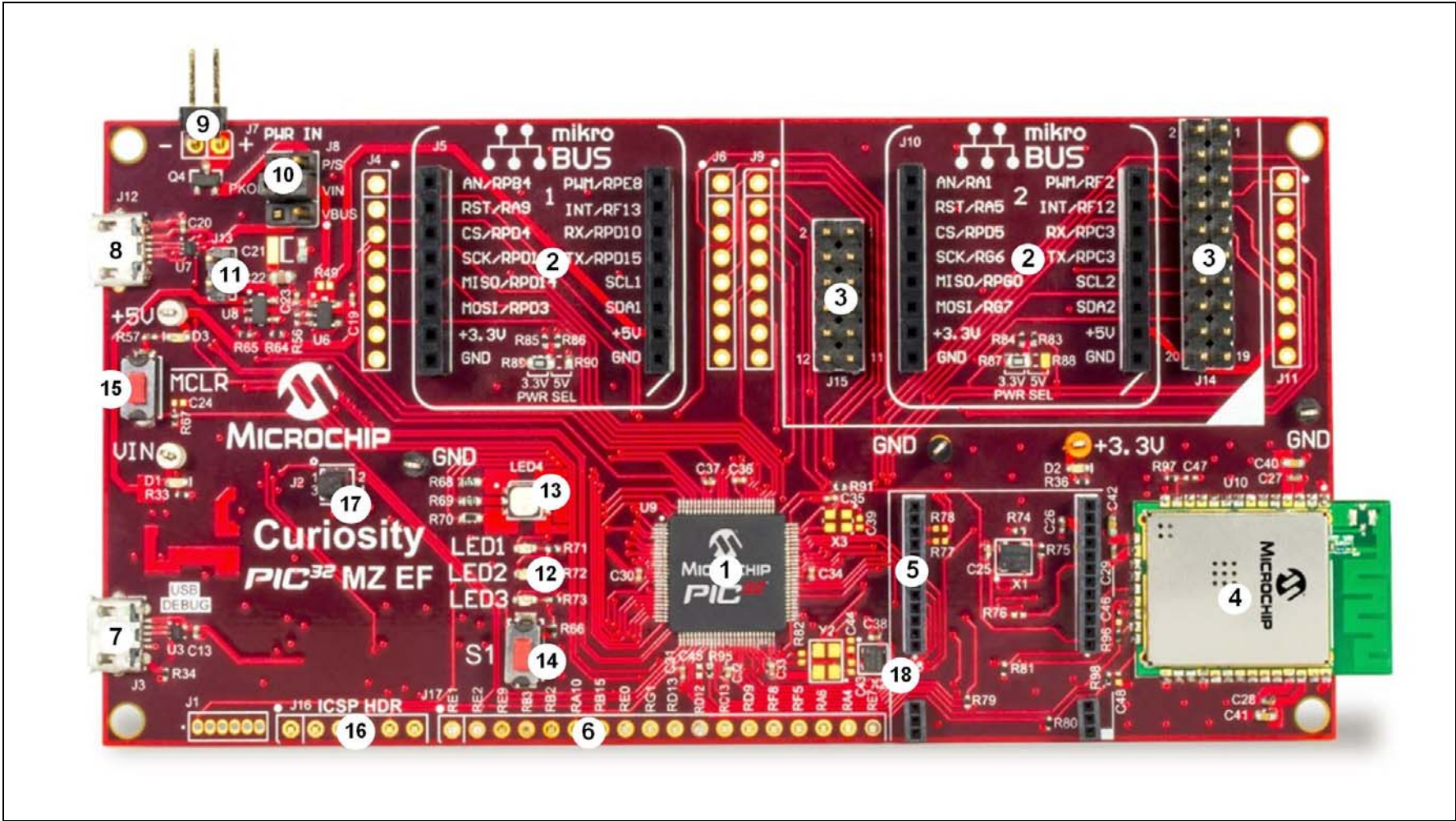
FIGURE 1-1: PIC32MZ EF CURIOSITY DEVELOPMENT BOARD LAYOUT (TOP VIEW)
