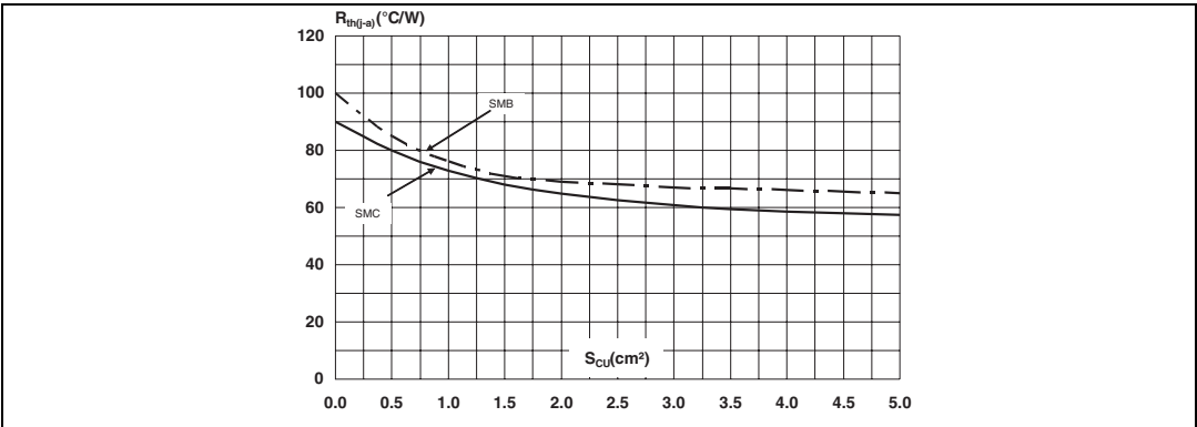
Figure 17. Thermal resistance junction to ambient versus copper surface under each lead, SMB, SMC (epoxy FR4, copper thickness = 35 µm)
