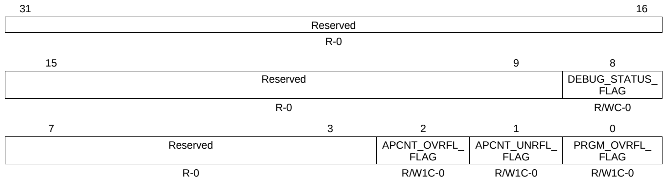
Figure 21-64. Exception Control Register 2 (HETEXC2)
