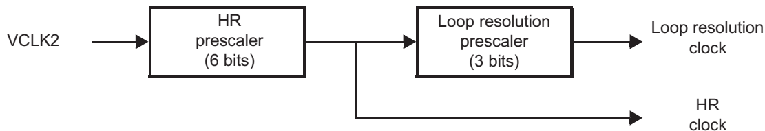
Figure 21-7. Prescaler Configuration
