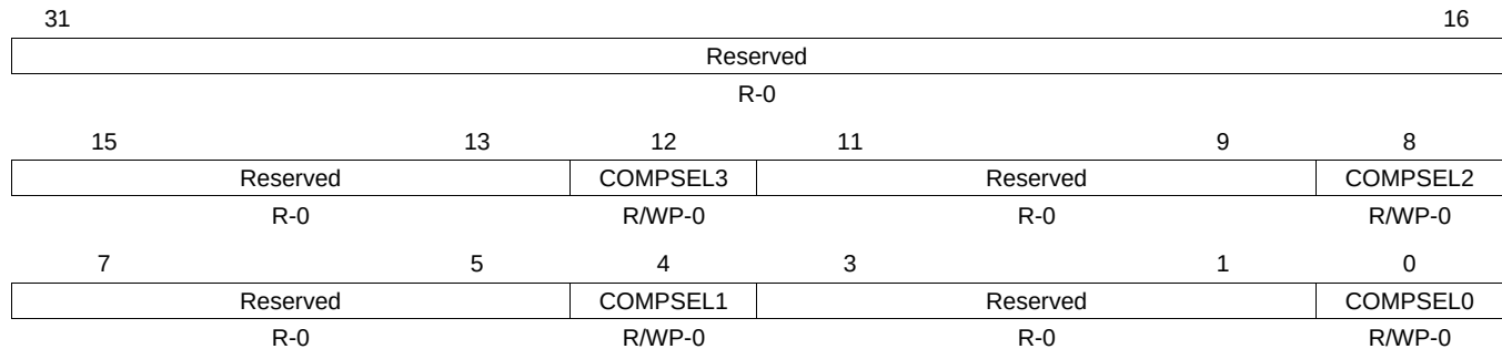
Figure 13-11. RTI Compare Control Register (RTICOMPCTRL) [offset = 0Ch]
