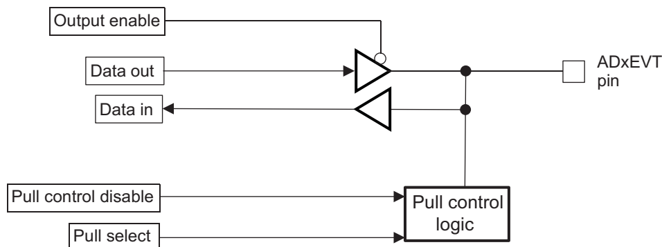
Figure 20-19. GPIO Functionality of ADxEVT
