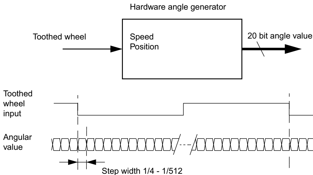
Figure 21-35. Angle Generator Principle
