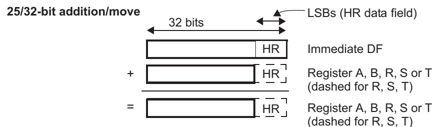
Figure 21-126. ADM32 Add and Move Operation for IM&REGTOREG (Case 00)
