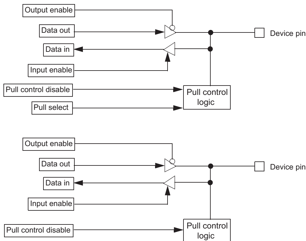
Figure 26-60. GPIO Functionality
