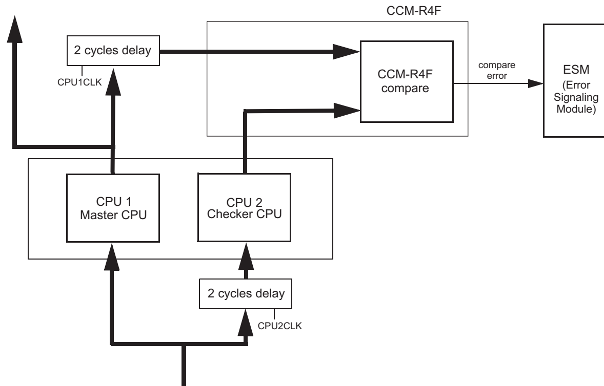
Figure 9-1. Block Diagram
