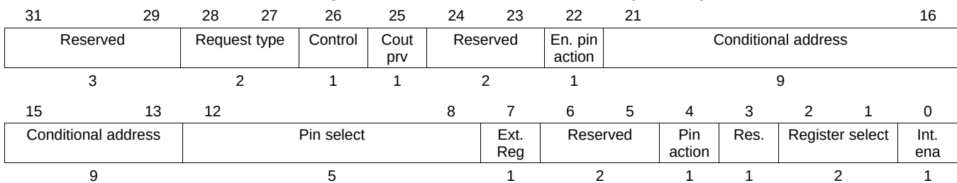
Figure 21-110. ACMP Control Field (C31:C0)
