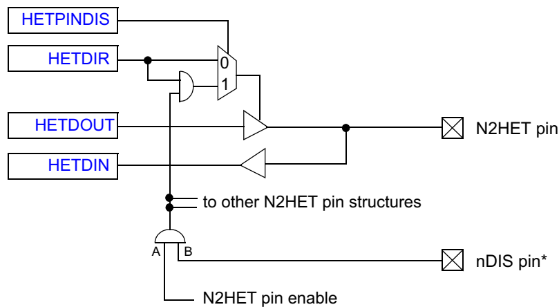
Figure 21-25. N2HET Pin Disable Feature Diagram
