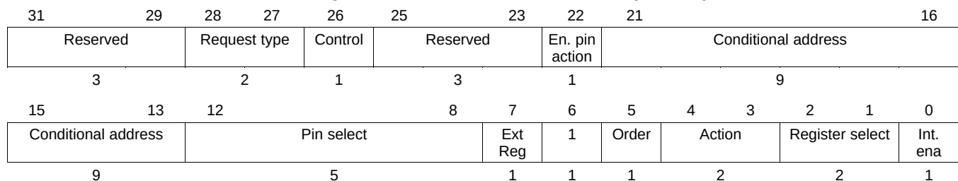
Figure 21-151. MCMP Control Field (C31:C0)
