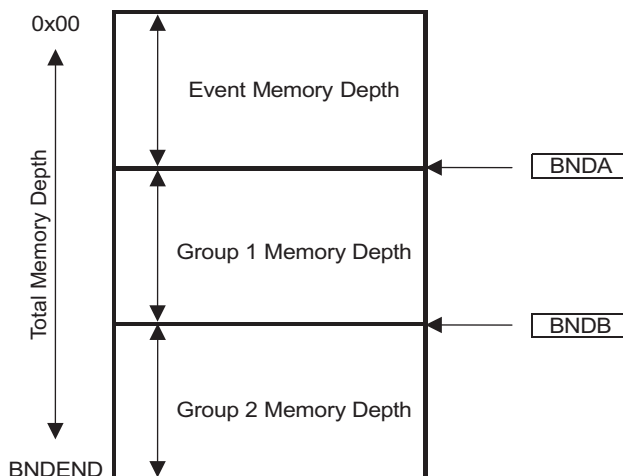
Figure 20-3. FIFO Implementation
