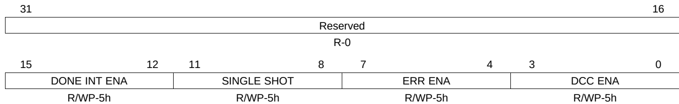
Figure 11-7. DCC Global Control Register (DCCGCTRL) [offset = 00]
