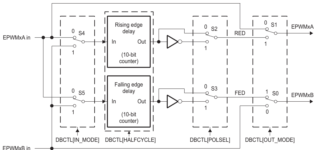
Figure 17-28. Configuration Options for the Dead-Band Submodule
