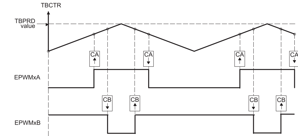
Figure 17-25. Up-Down-Count, Dual Edge Symmetric Waveform, With Independent Modulation on EPWMxA and EPWMxB — Complementary
