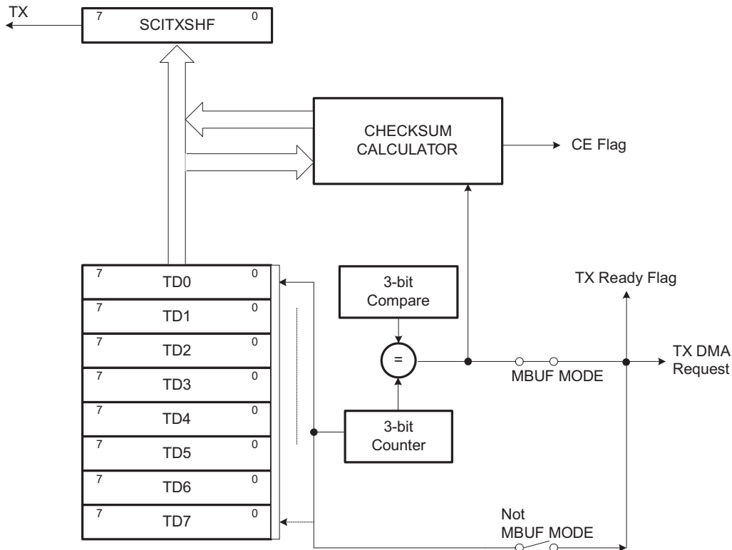
Figure 26-9. Transmit Buffers
