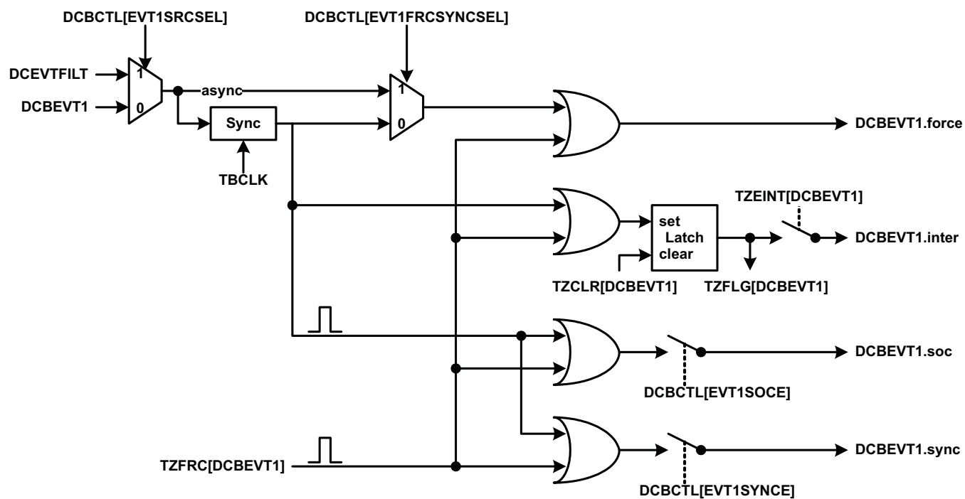
Figure 17-47. DCBEVT1 Event Triggering
