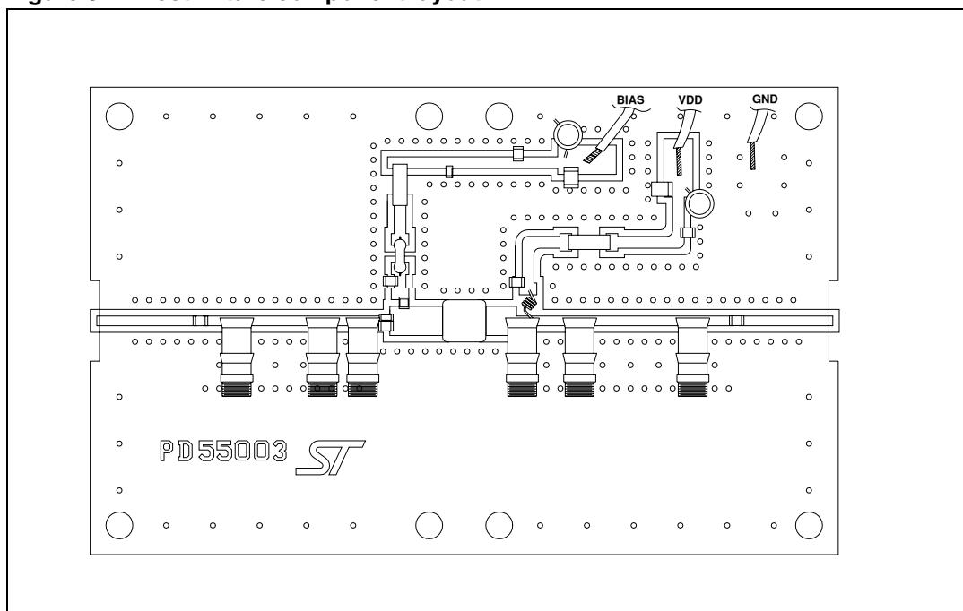
Figure 33. Test circuit photomaster
