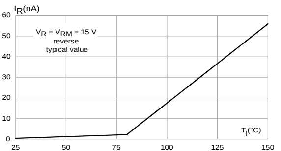
Figure 6: Leakage current versus junction temperature (typical value)
