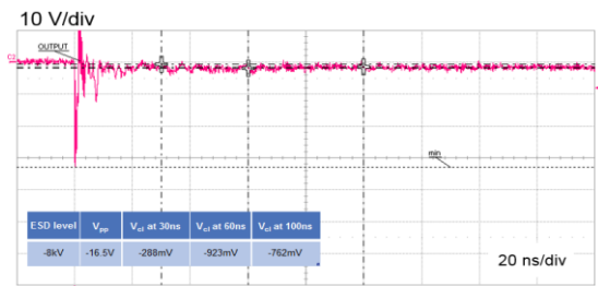
Figure 8: ESD response to IEC 61000-4-2 (-8kV contact discharge)
