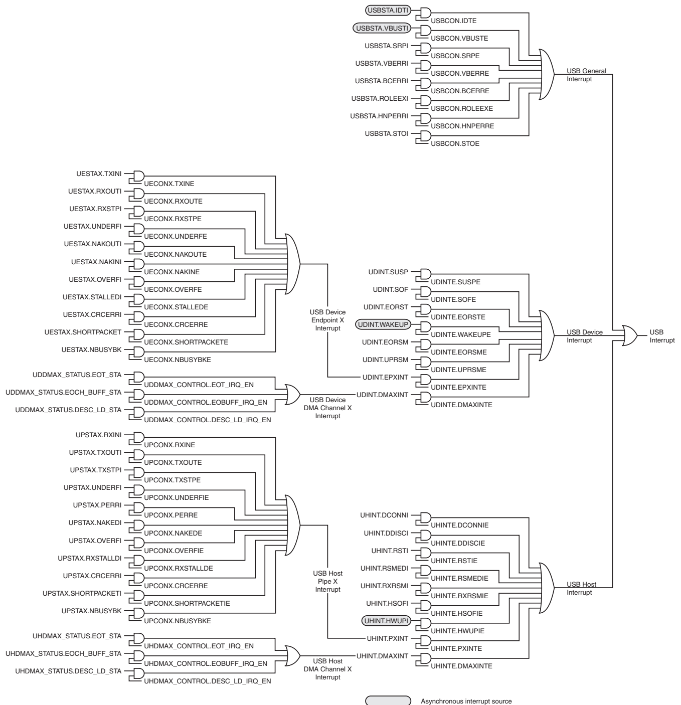
Figure 22-6. Interrupt System
