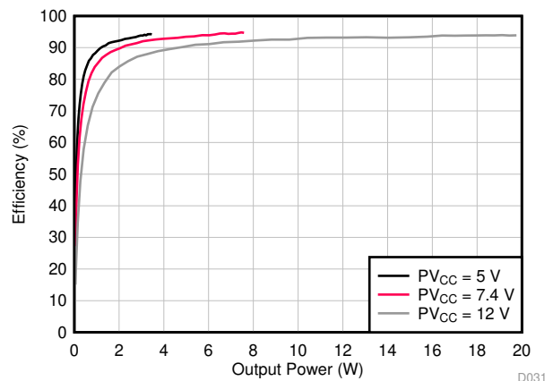
Figure 31. Efficiency vs Output Power, 4 \Omega
