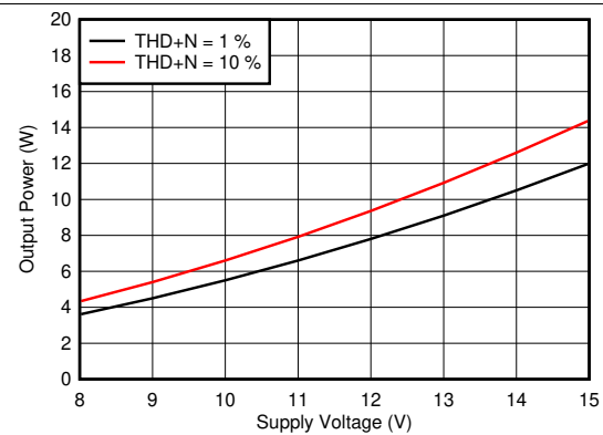
Load = 8 \Omega
