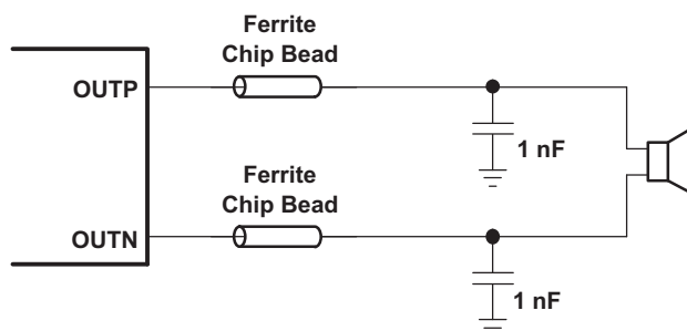
Figure 38. Typical Ferrite Chip Bead Filter (Chip Bead Example: NFZ2MSM series from Murata)
