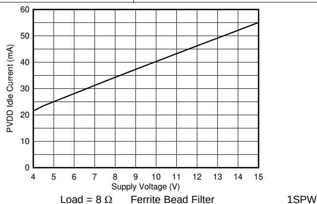
Figure 23. Idle Current vs Supply Voltage
