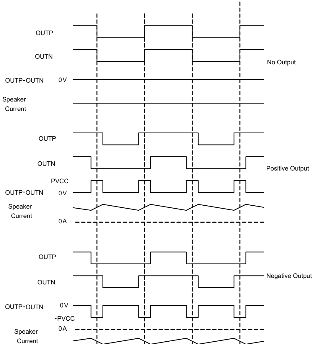
Figure 34. BD Mode Modulation
