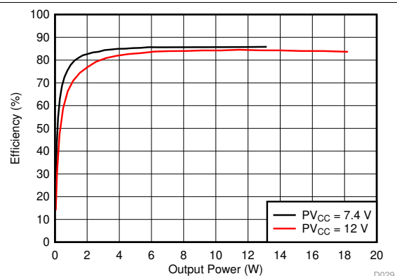
Figure 20. Efficiency vs Output Power, 4 \Omega
