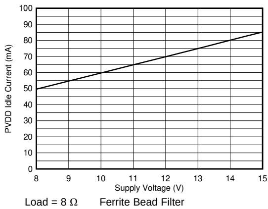
Figure 13. Idle Current vs Supply Voltage, 8 \Omega
