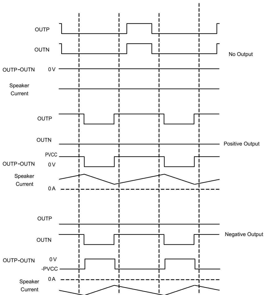
Figure 35. Low-Idle-Current 1SPW Modulation
