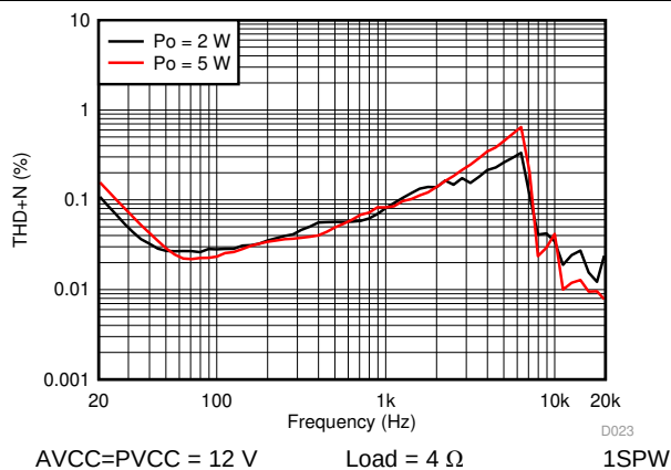
Figure 17. THD+N vs Frequency, 4 \Omega
