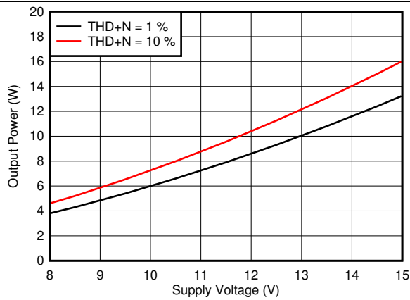
Figure 24. Output Power vs Supply Voltage, 8 \Omega
