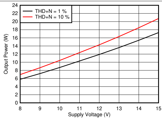
Load = 4 \Omega
