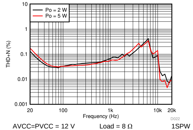
Figure 16. THD+N vs Frequency, 8 \Omega
