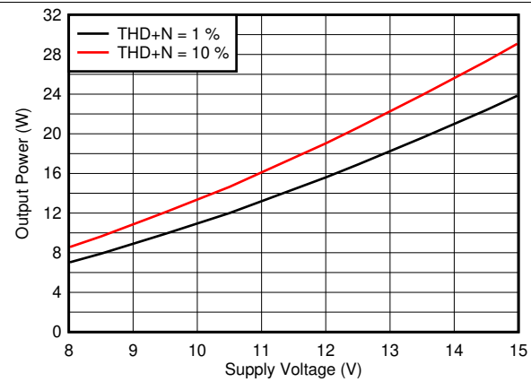
Figure 25. Output Power vs Supply Voltage, 4 \Omega
