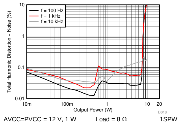
Figure 14. THD+N vs Output Power, 8 \Omega
