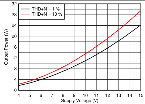
Figure 29. Output Power vs Supply Voltage, 4 \Omega
