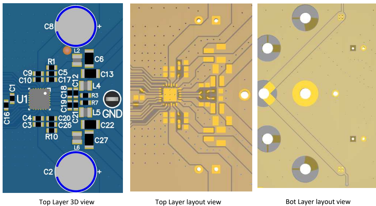
Figure 45. BTL Layout Example
