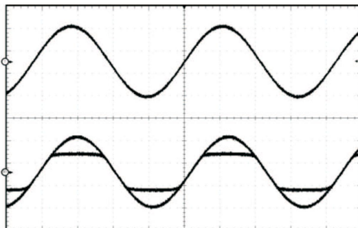
Figure 33. PLIMIT Circuit Operation
