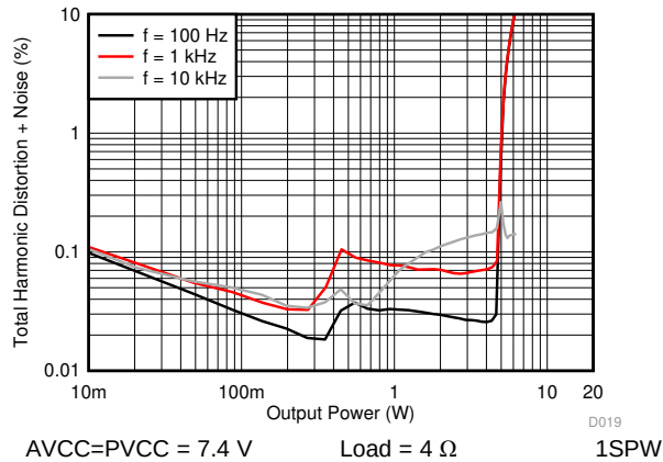
Figure 15. THD+N vs Output Power, 4 \Omega
