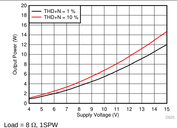
Figure 18. Output Power vs Supply Voltage, 8 \Omega
