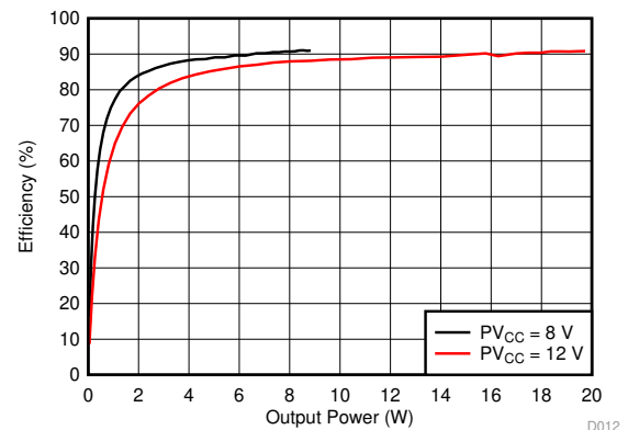
Figure 8. Efficiency vs Output Power (BTL)
