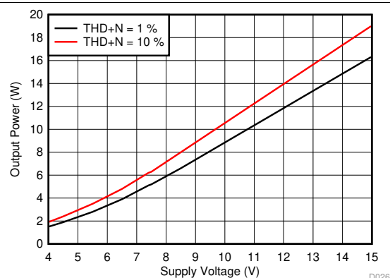
Figure 19. Output Power vs Supply Voltage, 4 \Omega
