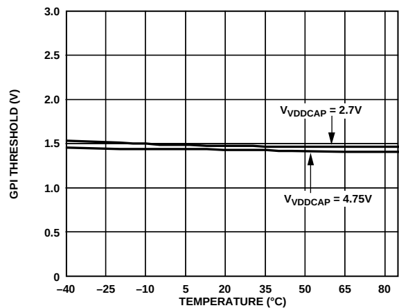
Figure 16. GPI Threshold vs. Temperature
