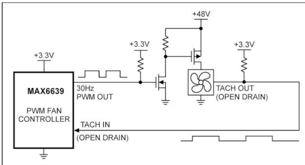
Figure 59. Controlling a 48V 2- or 3-wire fan by modulating the power supply with a PWM signal.
