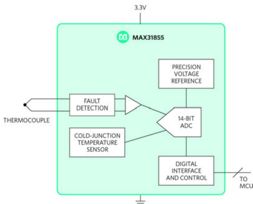
Figure 33. MAX31855 integrated thermocouple-to-digital converter with 3-wire interface.
