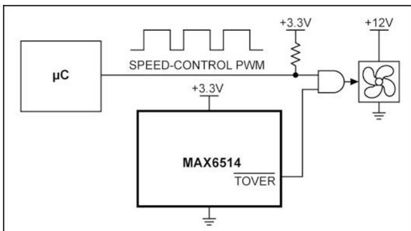
Figure 65. Fan fail-safe circuit with factory-set trip threshold
