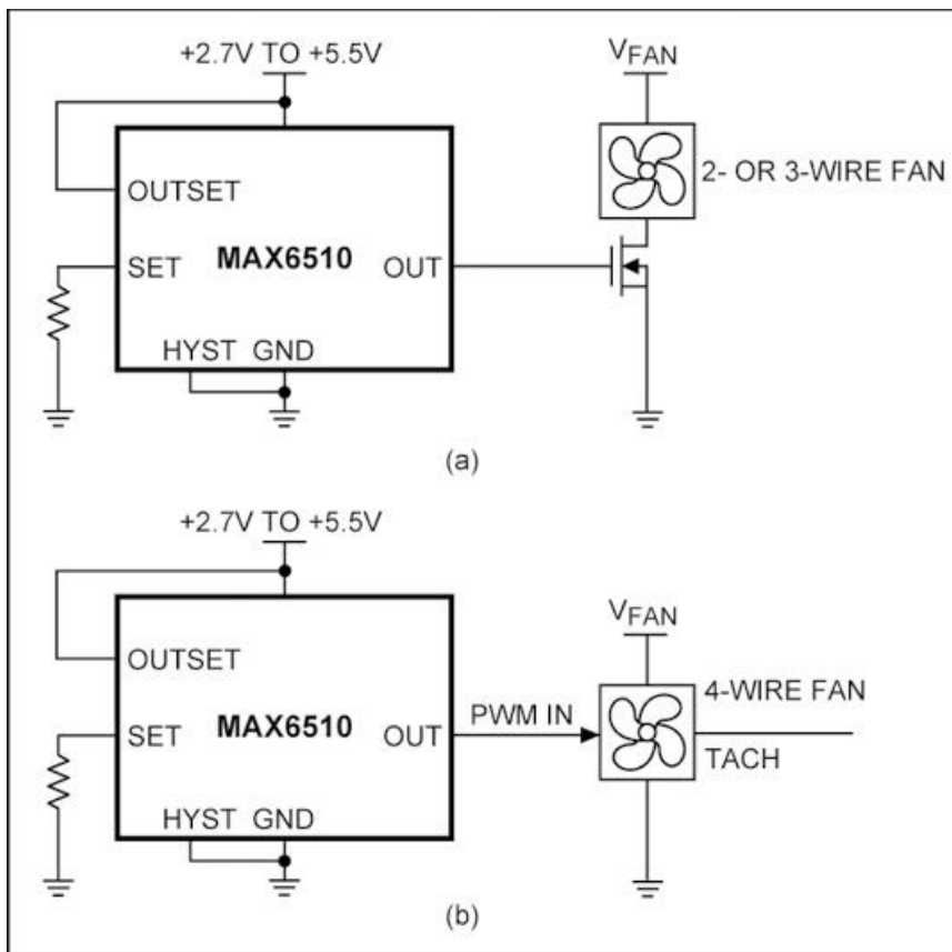
Figure 62. Local on/off fan controllers with adjustable thresholds. (a) Using a temperature switch and a FET to enable the fan's power supply for 2- and 3-wire fans. (b) The temperature switch's output directly drives a 4-wire fan's PWM input to activate the fan. The external resistor sets the trip threshold.
