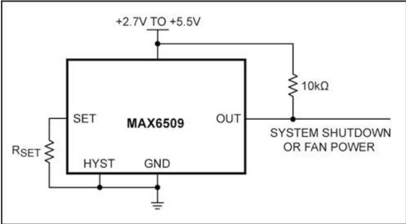
Figure 20. Temperature switch with a resistor-set trip temperature.
