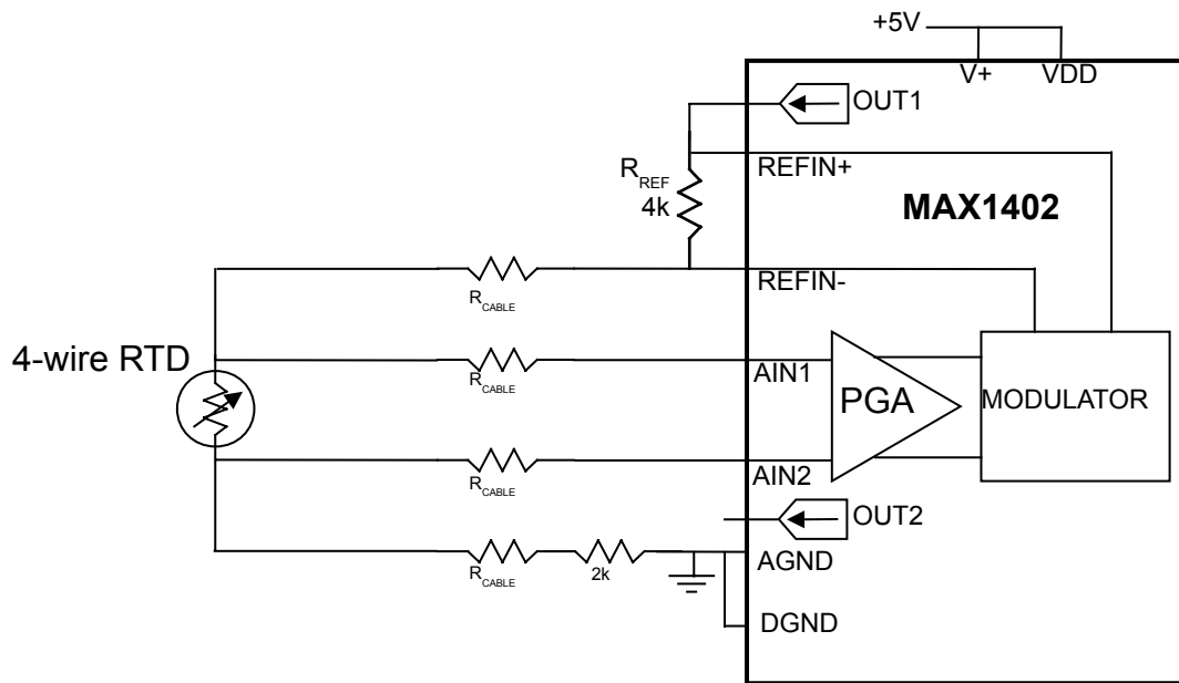
Figure 41a. 4-wire interface for a PT100 or PT1000 RTD.
