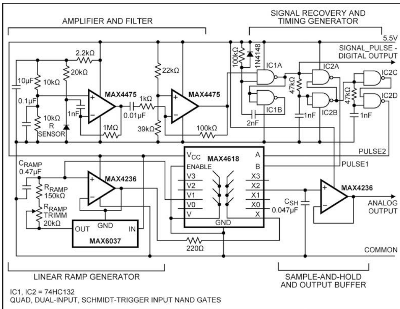
Figure 46. IR-linked temperature sensor. (a) Sensor and transmitter. (b) Receiver.
