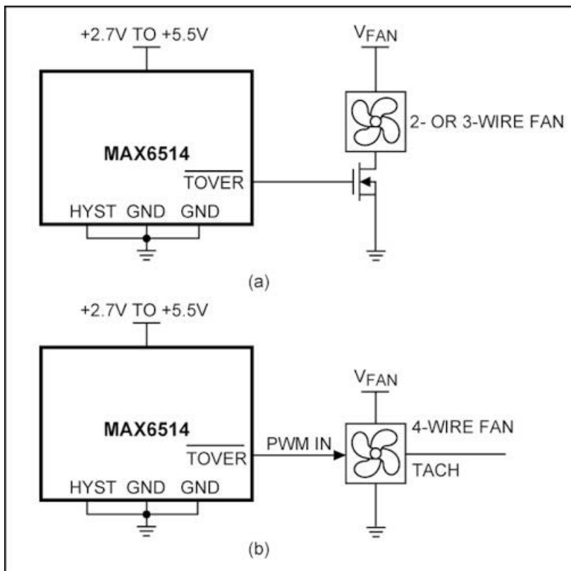
Figure 61. Local on/off fan controllers with factory-set thresholds. (a) Uses a temperature switch and a FET to enable the fan's power supply for 2- and 3-wire fans. (b) The temperature switch's output directly drives a 4-wire fan's PWM input to activate the fan.
