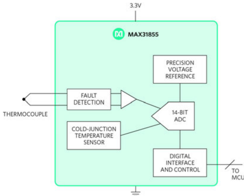
Figure 45a. Integrated thermocouple-to-digital converter with SPI interface. Versions are available for E, J, K, N, R, S, and T thermocouple types.
