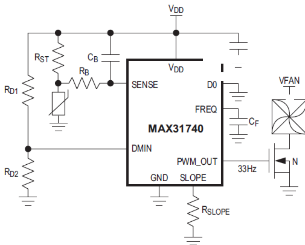
Figure 52a. Stand-alone speed controller for 2- or 3-wire fans.
