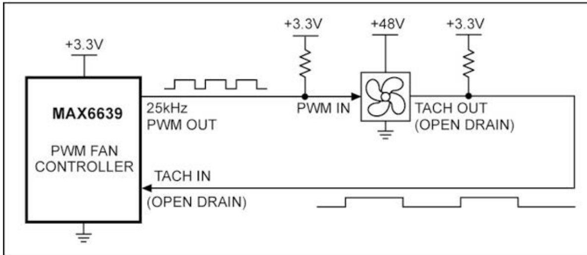
Figure 58. Controlling a 48V 4-wire fan. No special precautions are needed—any PWM-output fan controller with an appropriate output frequency available will work.
