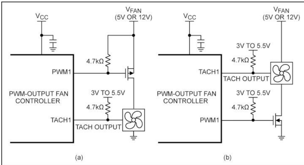
Figure 53. 3-wire fan control circuits using pulse-width modulation of the fan's power supply. 2-wire fans can be controlled with the same circuits, but do not have tachometer outputs. (a) High-side drive. (b) Low-side drive.
