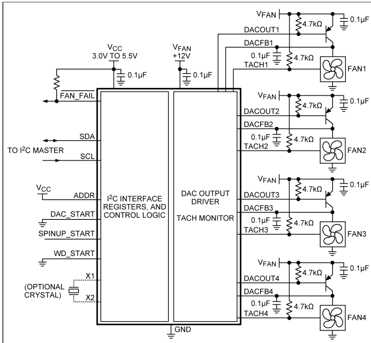
Figure 57. The MAX6620 shown here is a 4-channel linear fan speed controller using external pass transistors to supply variable power to the fans.
