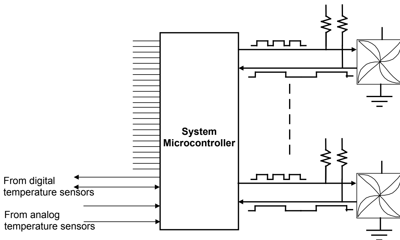
Figure 48. When sufficient I/Os are available and the fans are located nearby, an existing system management microcontroller may be used for fan speed control.
