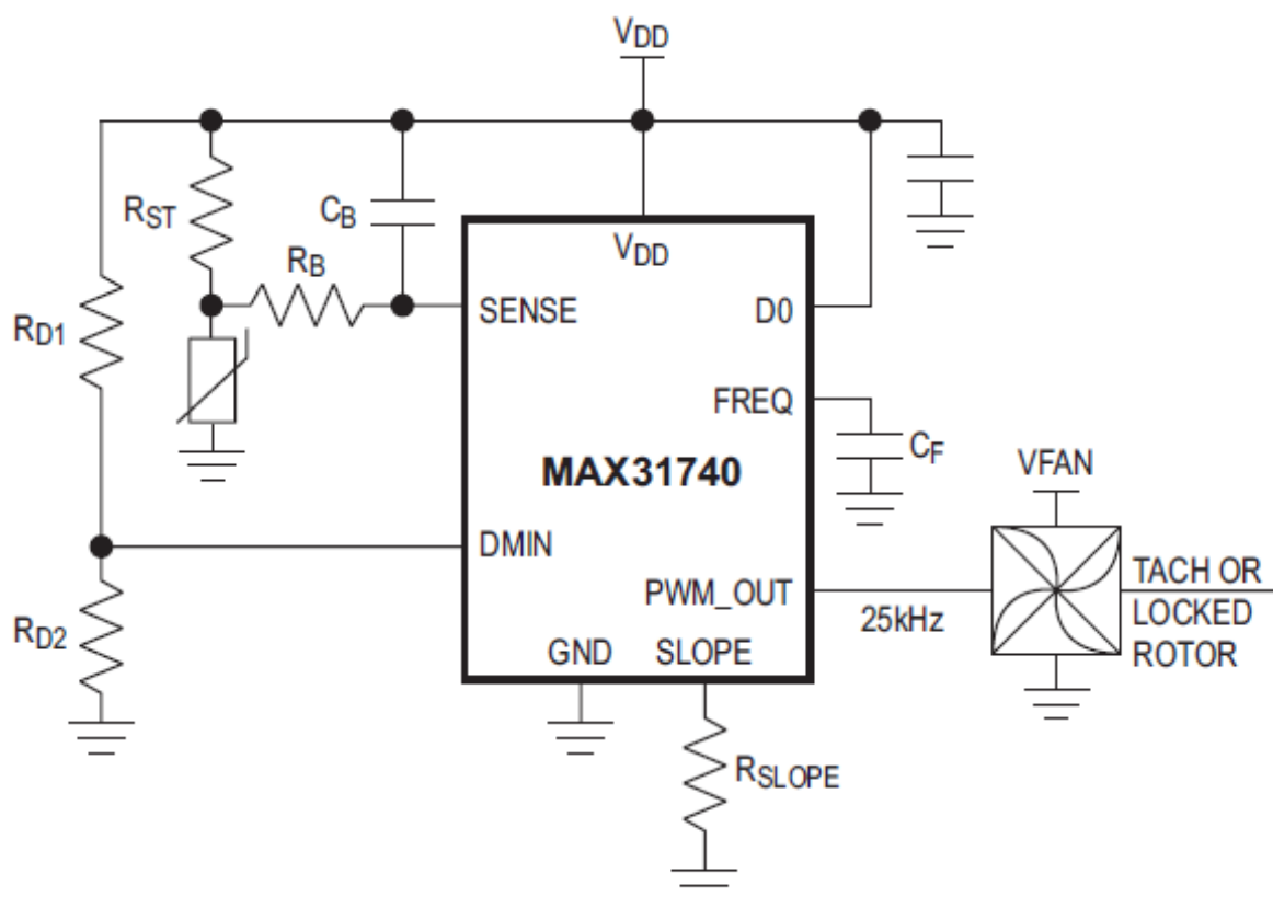
Figure 52b. Stand-alone speed controller for 4-wire fans or other fans with speed-control inputs. The TACH or locked-rotor output (if available) is not used by the MAX31740.
