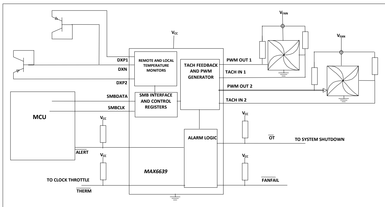
Figure 51. An automatic fan speed control IC like the MAX6639 monitors temperature and controls fan speed using parameters selected by the system microcontroller.
