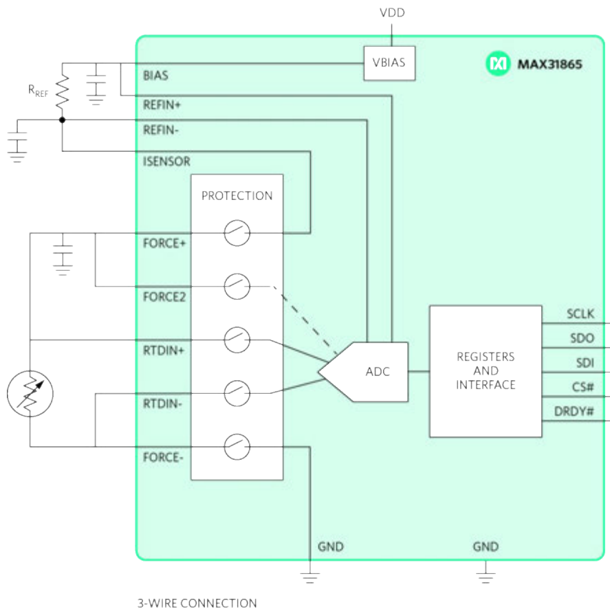
Figure 32. The MAX31865 digitizes the resistance of a 2-, 3-, or 4-wire RTD, detects cable and sensor faults, and includes \pm 45\text{V} input protection.
