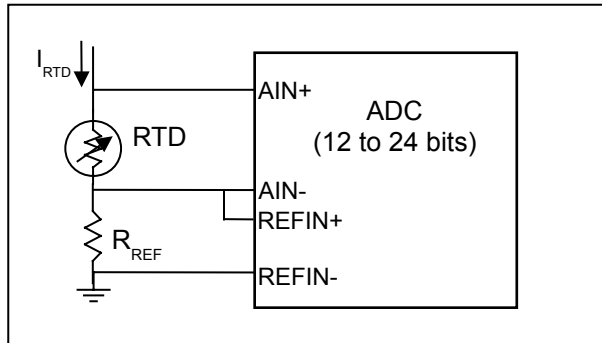
Figure 6. Simplified RTD signal-conditioning circuit.
