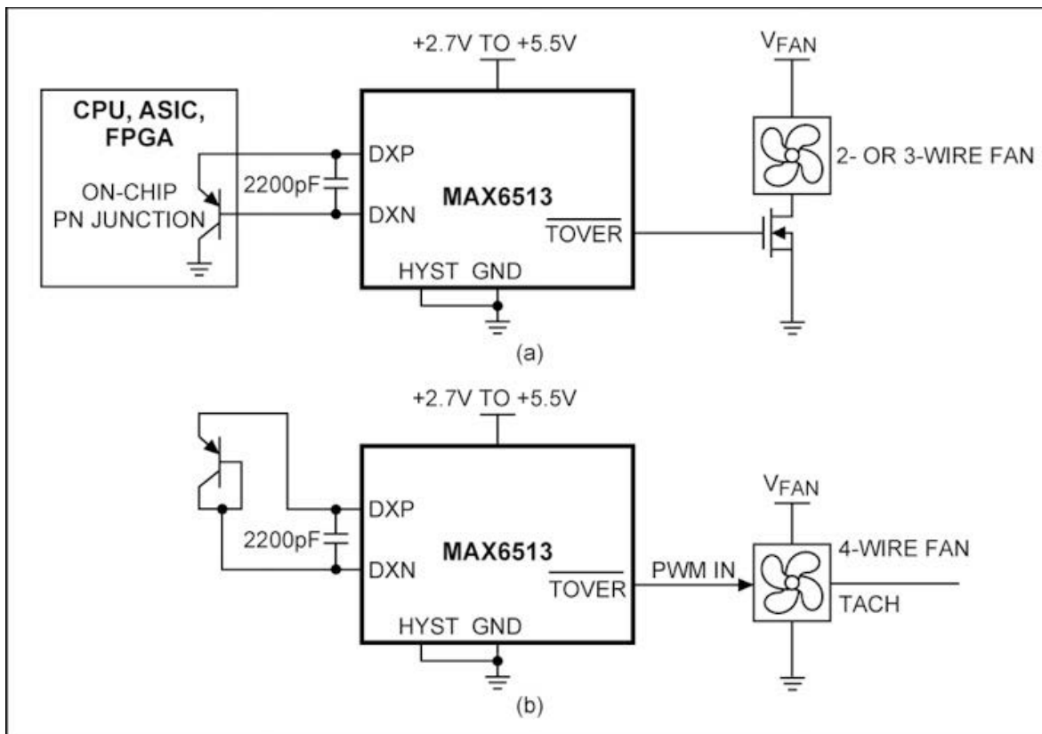
Figure 63. Remote, on/off fan controllers with factory-set thresholds. (a) Uses a remote temperature switch and a FET to enable the fan's power supply for 2- and 3-wire fans. (b) The temperature switch's output directly drives a 4-wire fan's PWM input to activate the fan.
