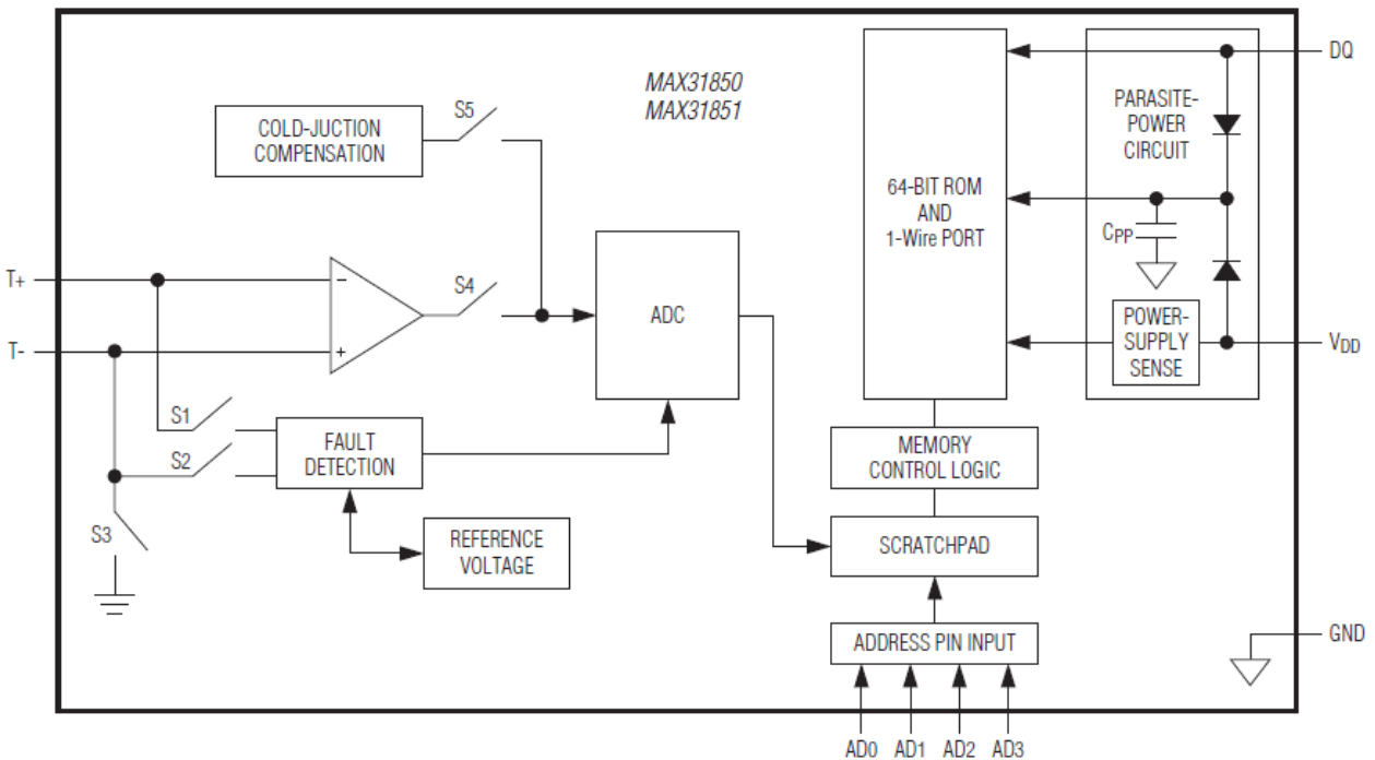
Figure 45b. Block diagram of the MAX31850 and MAX31851 1-Wire thermocouple-to-digital ICs.
