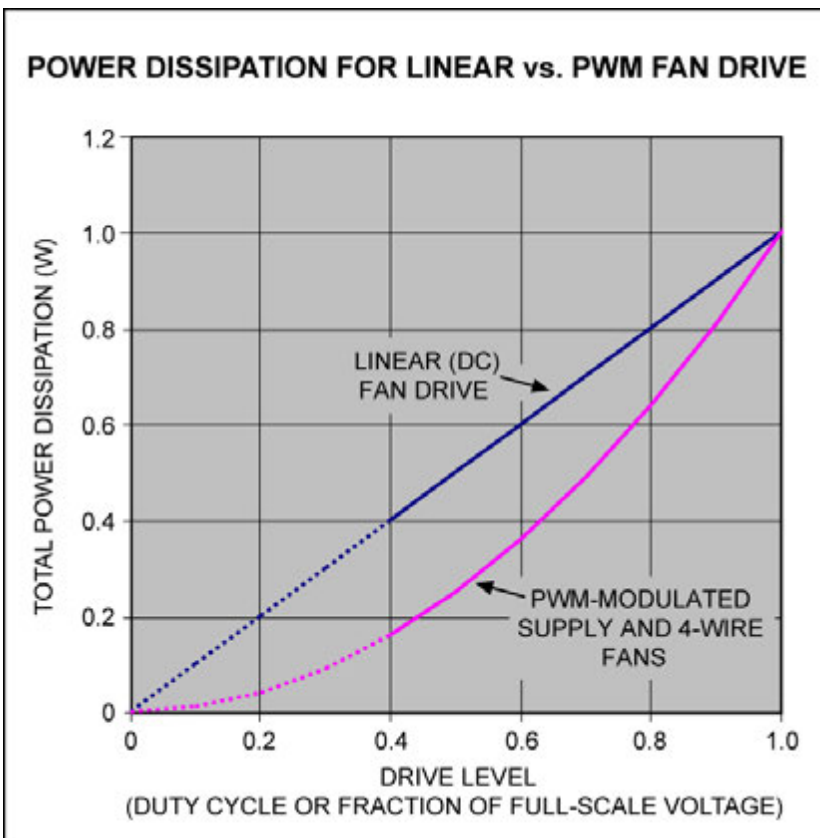
Figure 24. Comparison of power dissipation in linear (upper curve) and PWM fan drive (lower curve) approaches.
