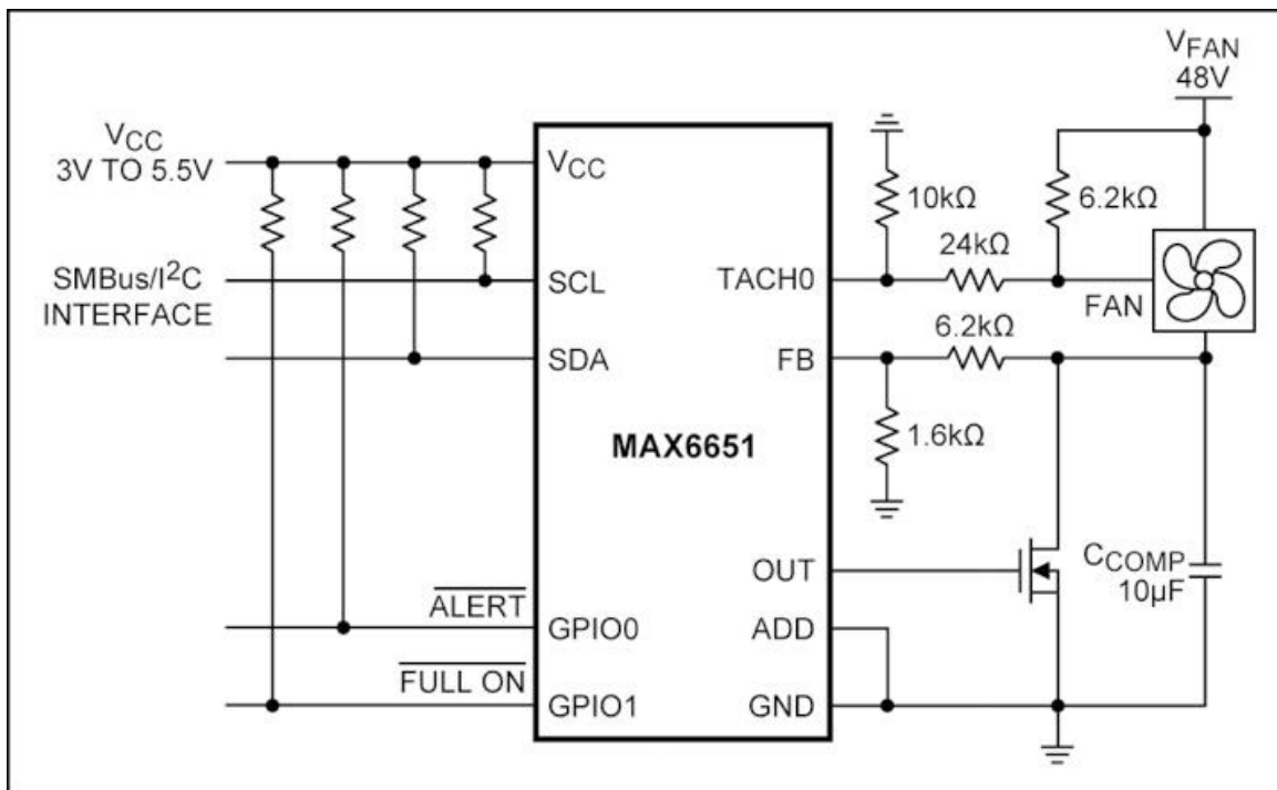
Figure 60. 48V, linear fan RPM controller. The feedback and tachometer signals are attenuated for compatibility with the MAX6651's input voltage tolerance.
