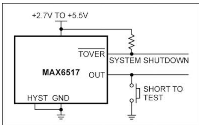
Figure 66. A simple way to verify temperature switch operation at the board level is to short the analog voltage output to ground. This makes the temperature switch react as though the temperature is high: the active-low TOVER output trips, thus verifying functionality.
