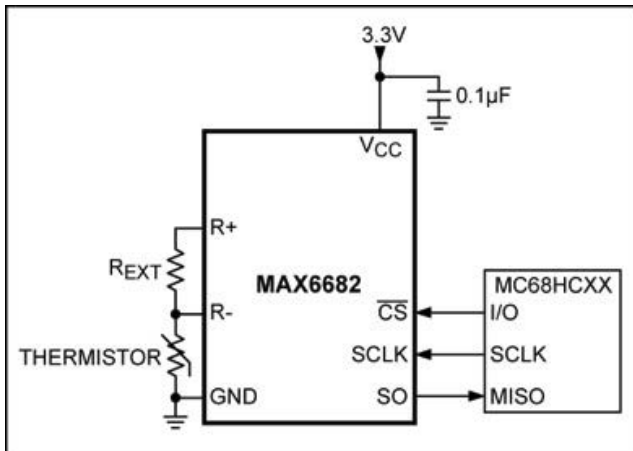
Figure 31. MAX6682 single thermistor-to-digital converter.
