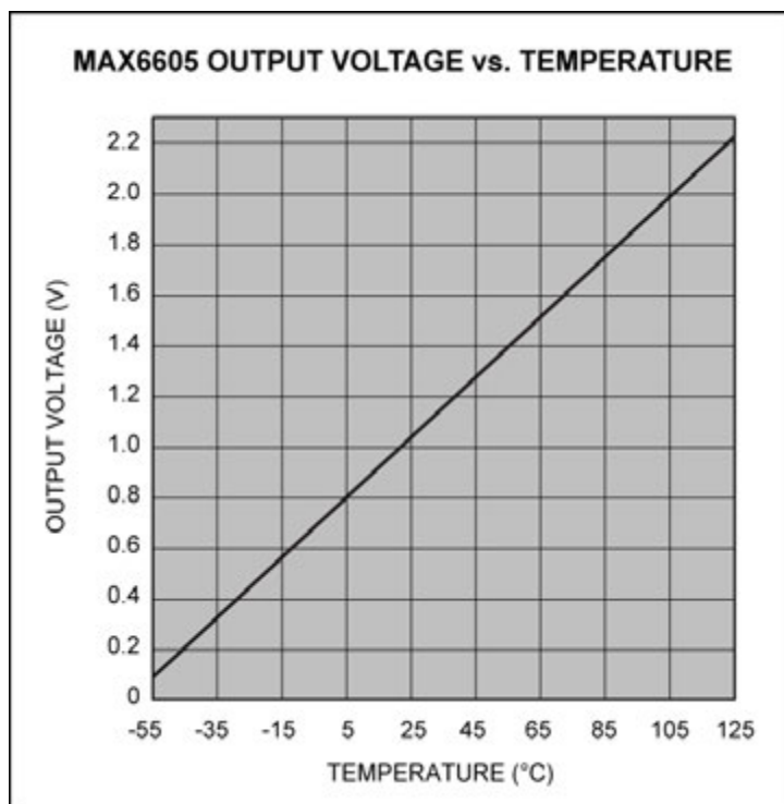
Figure 12. Output voltage vs. temperature for the MAX6605 analog temperature-sensor IC.
