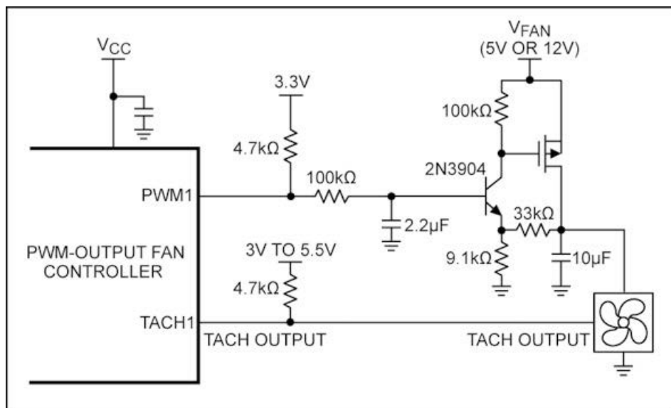
Figure 55. Circuit for converting PWM fan control signals to a linear supply voltage.
