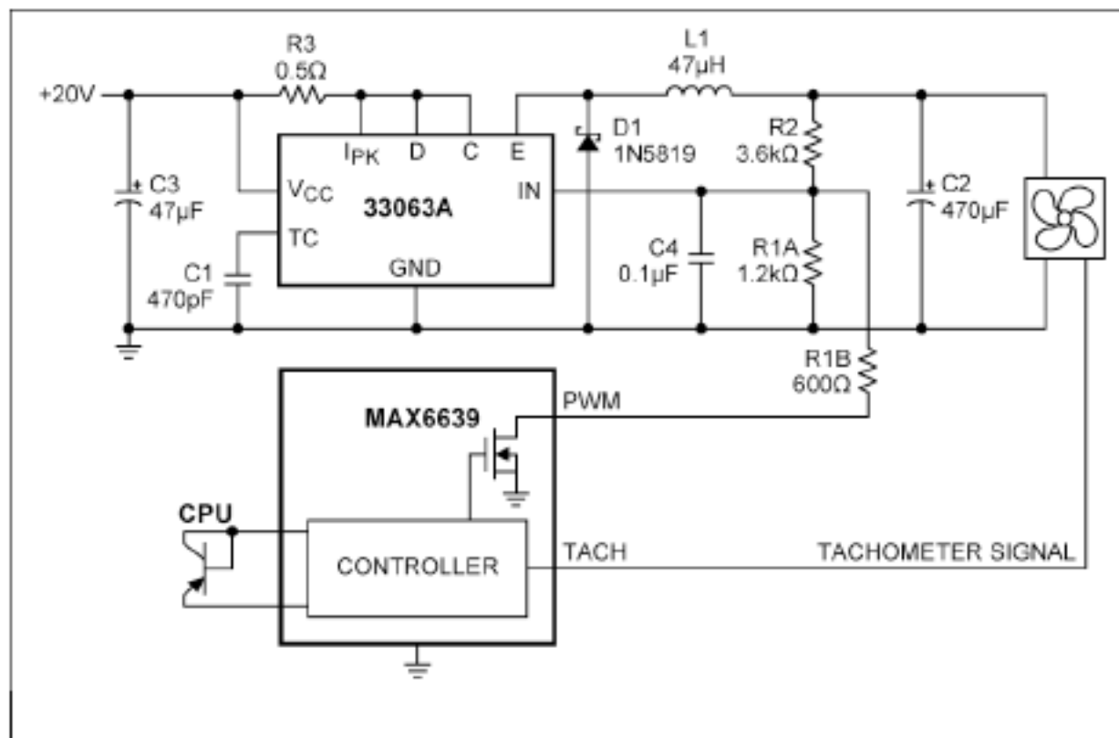
Figure 56. Linear drive from a PWM-output fan controller using an external switch-mode voltage regulator.
