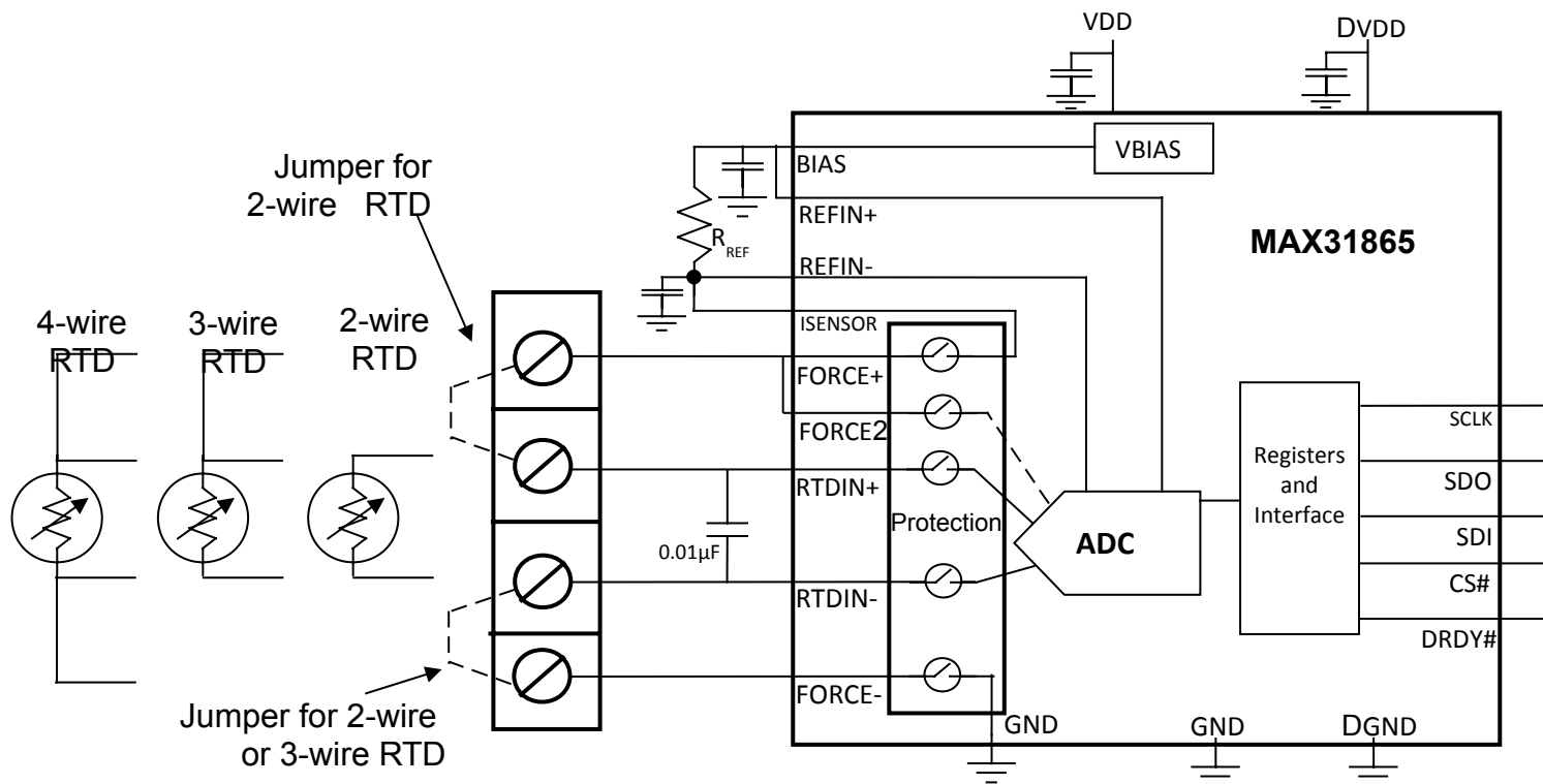
Figure 41c. 2-, 3-, and 4-wire interface for PT100 or PT1000 RTDs using the MAX31865 RTD digitizer.
