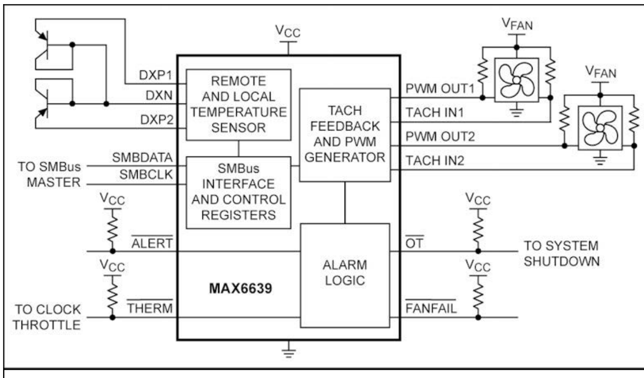
Figure 54. The MAX6639 controlling two 4-wire fans; it measures two temperatures and can control fan RPM based on the measured temperature.
