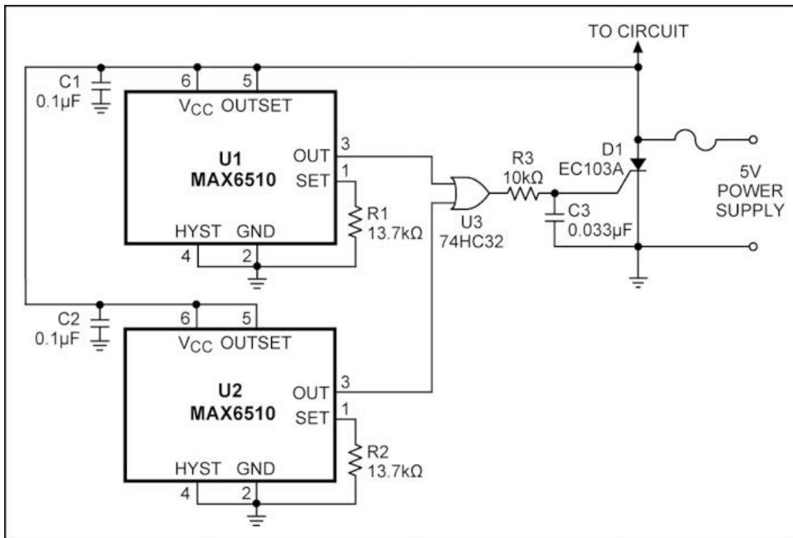
Figure 67. Overtemperature crowbar circuit with two temperature switches. If either temperature switch is hot enough to trip, SCR D1 will turn on, thus shorting the power supply and blowing the fuse.
