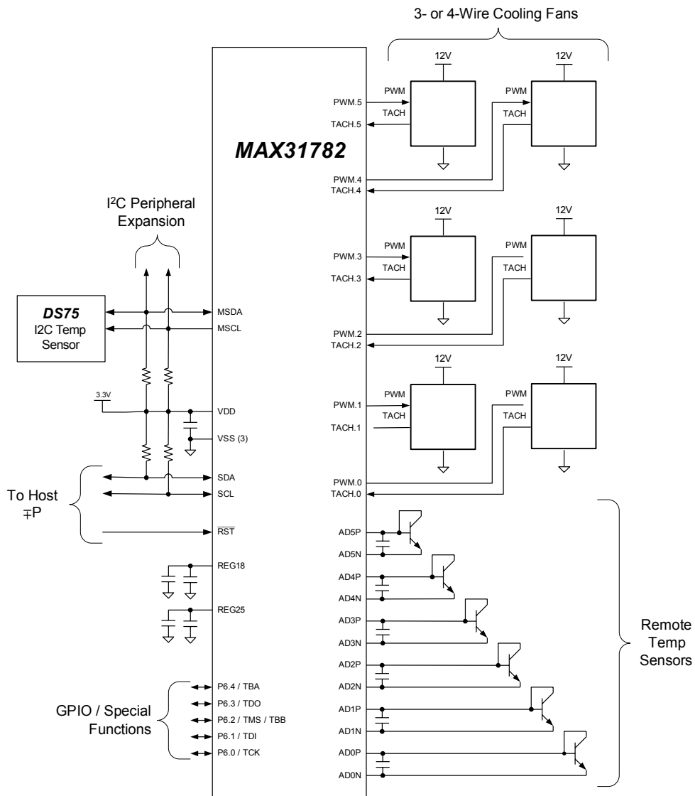
Figure 49. A dedicated Thermal Management Microcontroller monitors temperature from multiple sources and controls an array of fans in response to temperature data.
