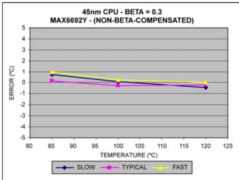
Figure 18. Three samples of a 45nm microprocessor with \beta = 0.3 measured using conventional MAX6692Y remote temperature sensors. Note the low errors even without beta compensation.
