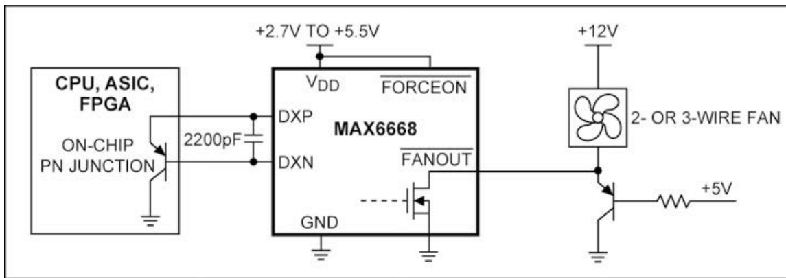
Figure 64. Remote, two-speed fan controller with factory-set threshold. Below the threshold, the fan runs at approximately half speed. Above the threshold, it runs at full speed.
