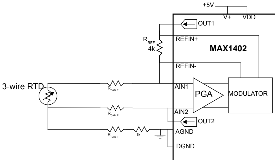
Figure 41b. 3-wire interface for a PT100 or PT1000 RTD.
