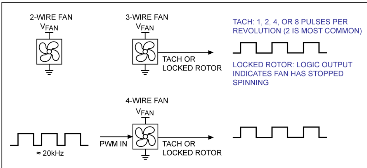
Figure 21. 2-, 3-, and 4-wire fans.
