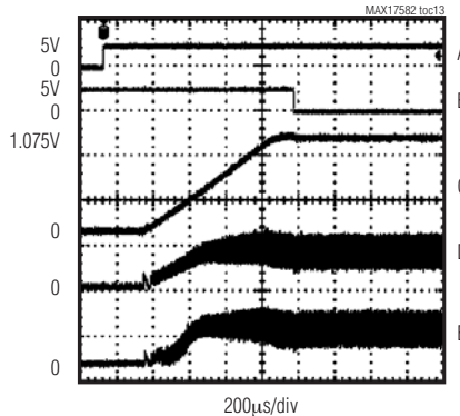
SOFT-START WAVEFORM (UP TO CLKEN)
