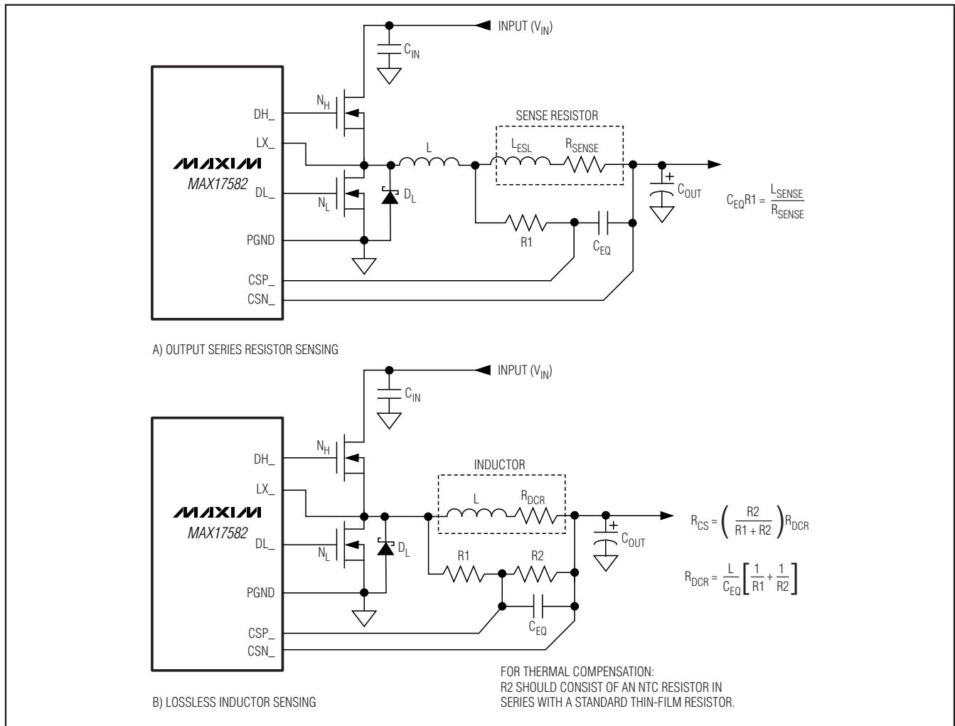
Figure 3. Current-Sense Methods
