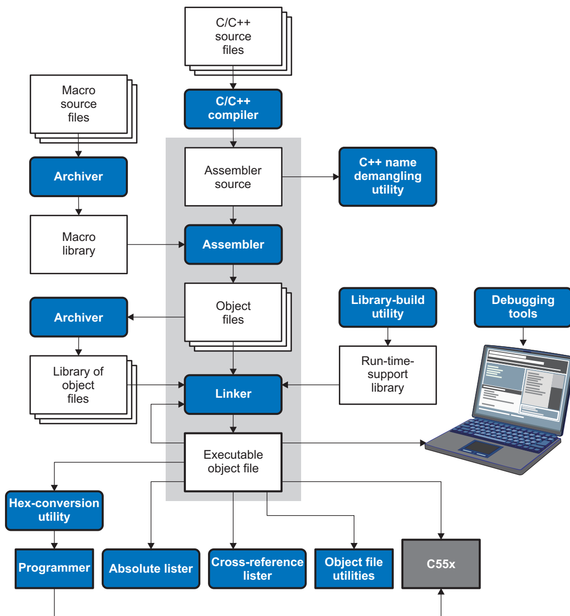
Figure 9-1. The Linker in the TMS320C55x Software Development Flow
