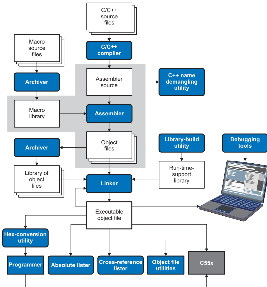
Figure 3-1. The Assembler in the TMS320C55x Software Development Flow
