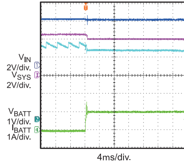
Battery Insertion
