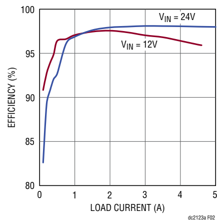
Figure 2. Efficiency
