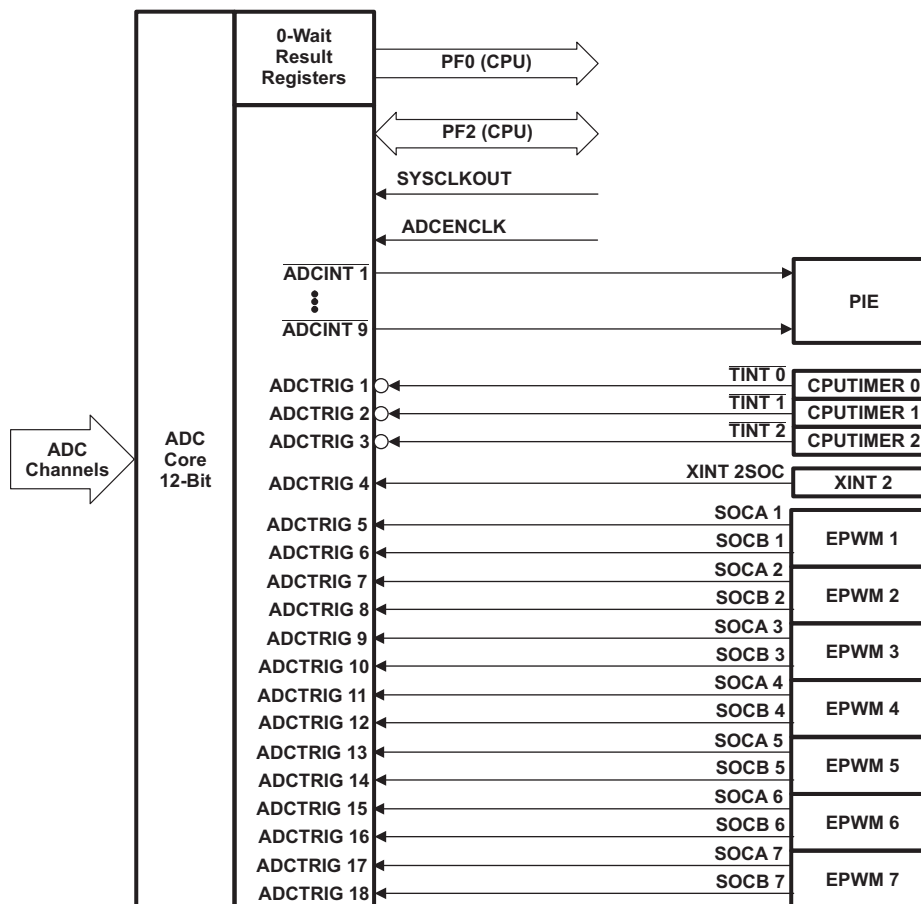
Figure 6-16. ADC Connections
