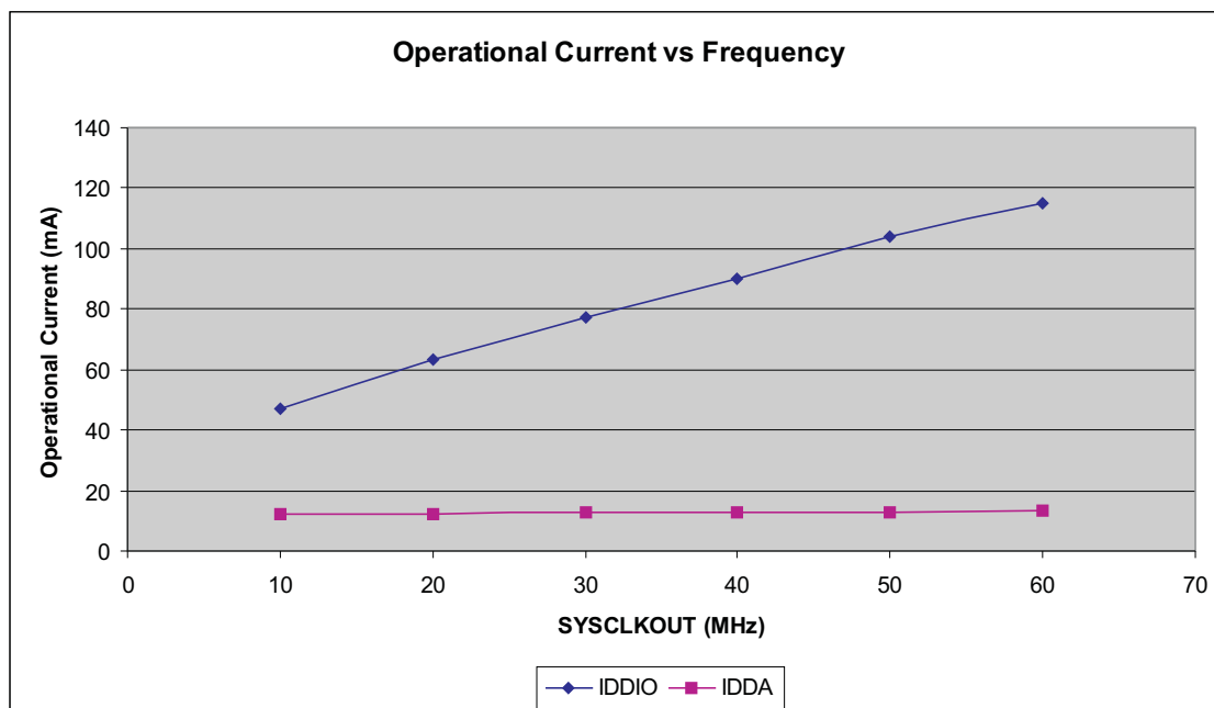
Figure 5-1. Typical Operational Current Versus Frequency (F2805x)
