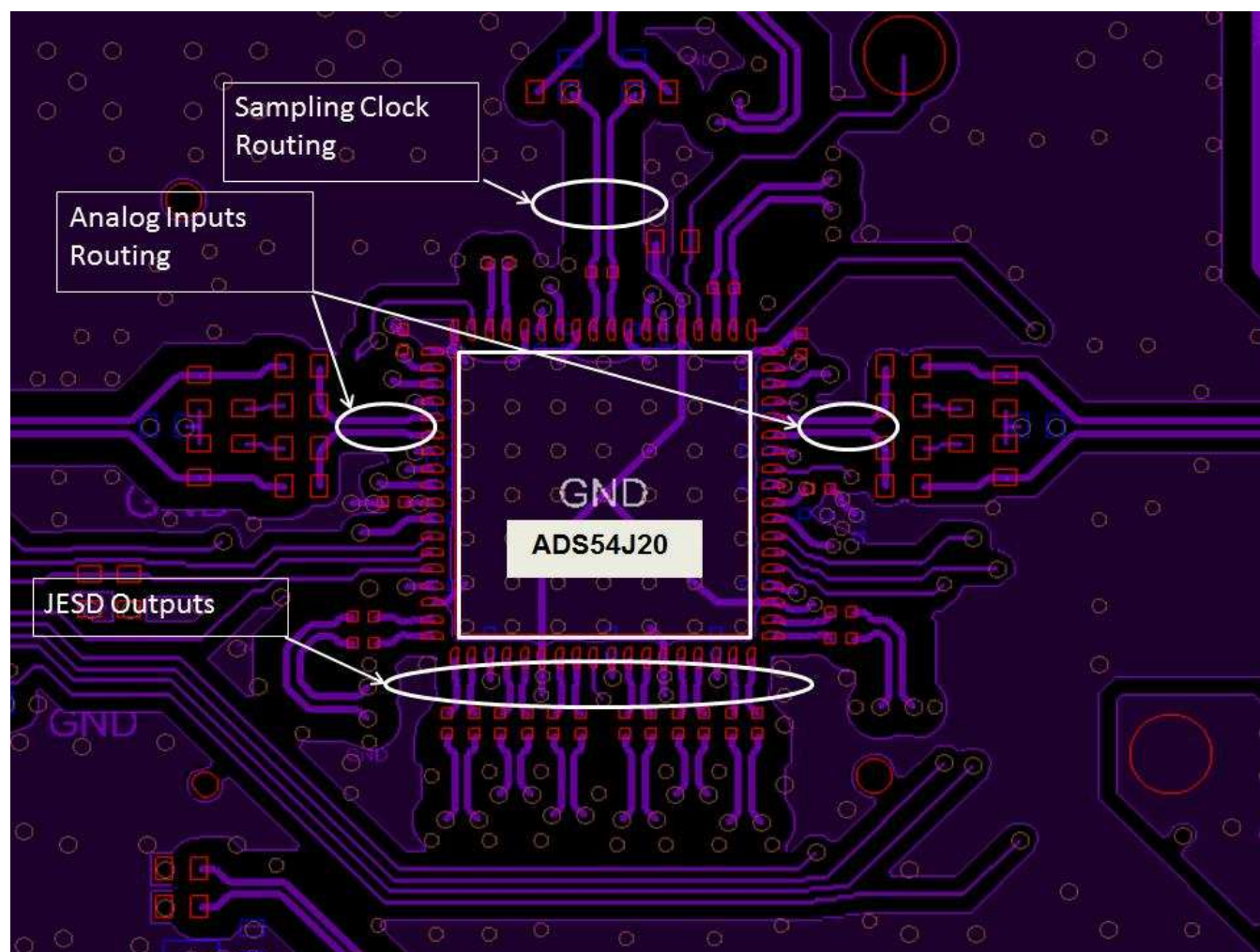
Figure 139. ADS54J20EVm Layout
