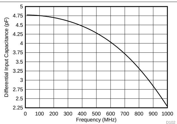
Figure 134. C_{IN} vs Input Frequency
