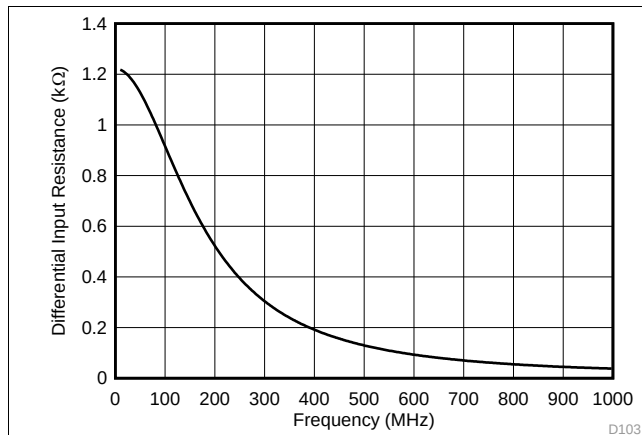
Figure 133. R_{IN} vs Input Frequency
