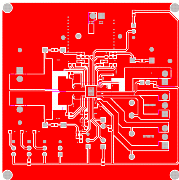
Figure 3. Top Layer
