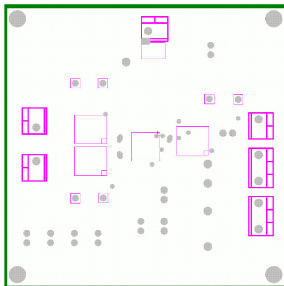
Figure 4. Middle Layer (2nd), Solid Cu Ground
