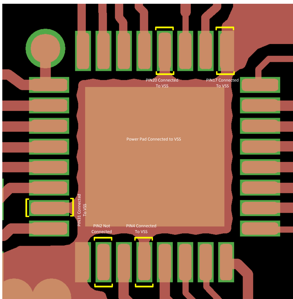
Figure 22. UCD9081 Layout, Top Layer
