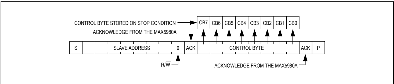
Figure 10. Write Format, Control Byte Received
