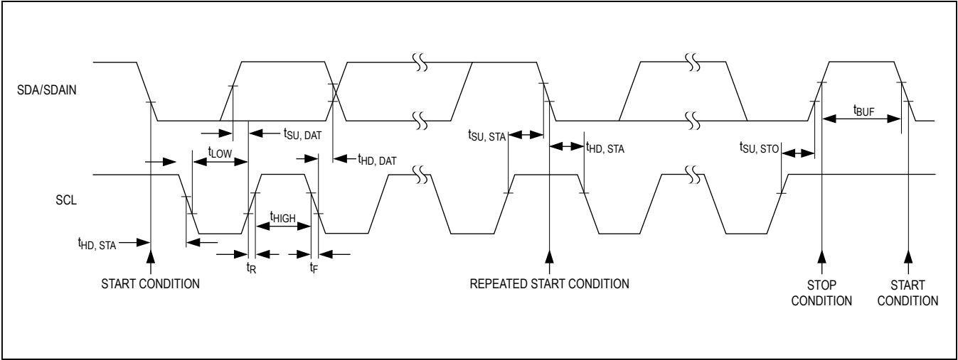
Figure 5. Serial Interface Timing Details
