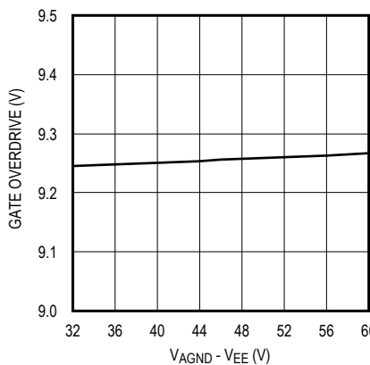
GATE OVERDRIVE VOLTAGE vs. ANALOG SUPPLY VOLTAGE
